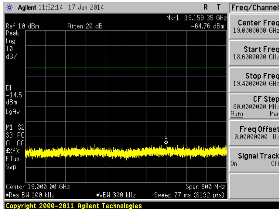
Plot 198 – Channel 6 (mid ch) @ DQPSK 2Mbps
