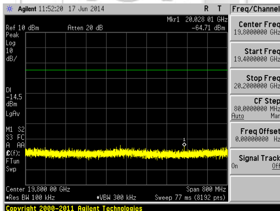
Plot 199 – Channel 6 (mid ch) @ DQPSK 2Mbps
