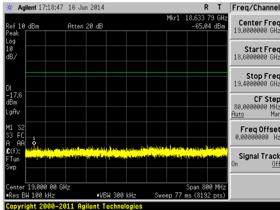
Plot 422 – Channel 1 (lower ch) @ 16QAM 36Mbps
