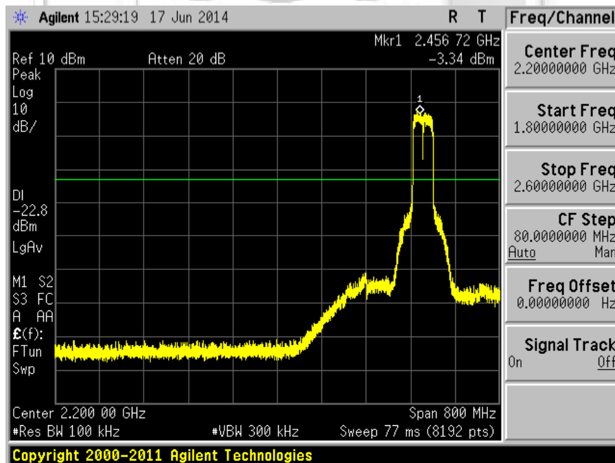
Plot 1425 – Channel 11 (upper ch) @ MCS12-162Mbps
