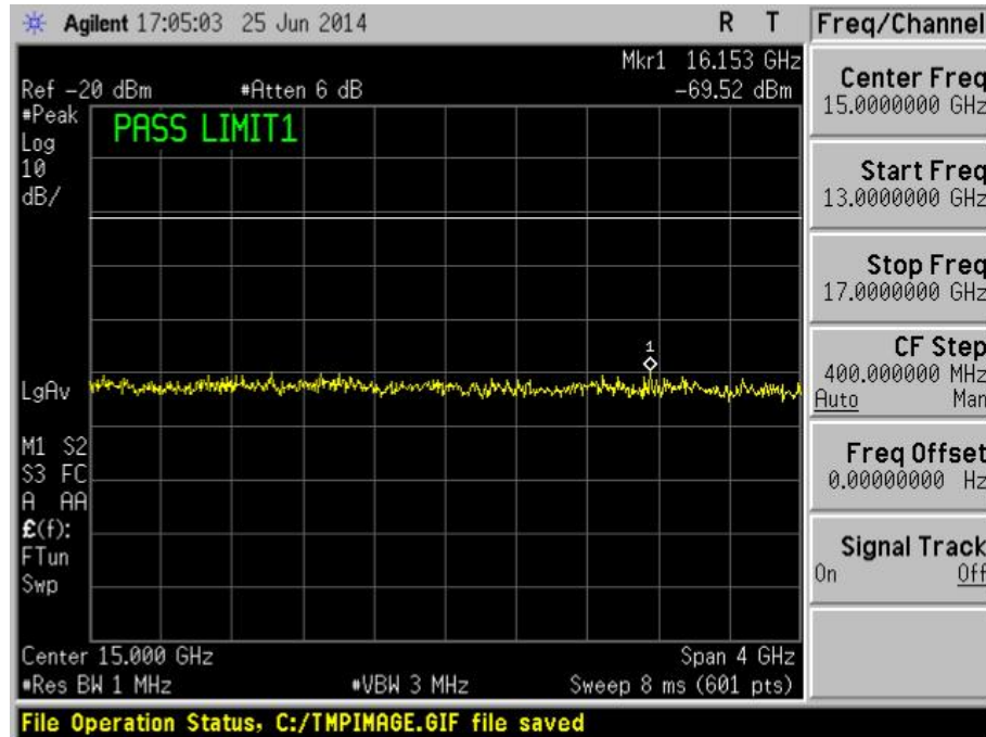
Plot 1753 – Channel 11 (upper ch) @ BPSK 13Mbps
