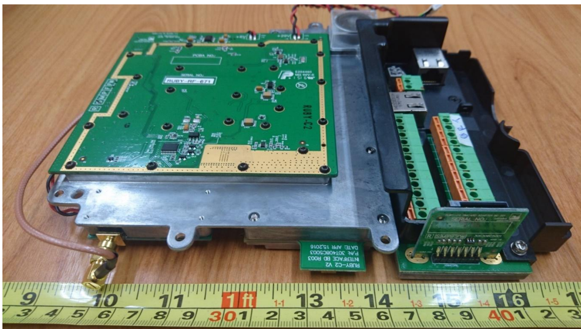
EUT Internal View 2
