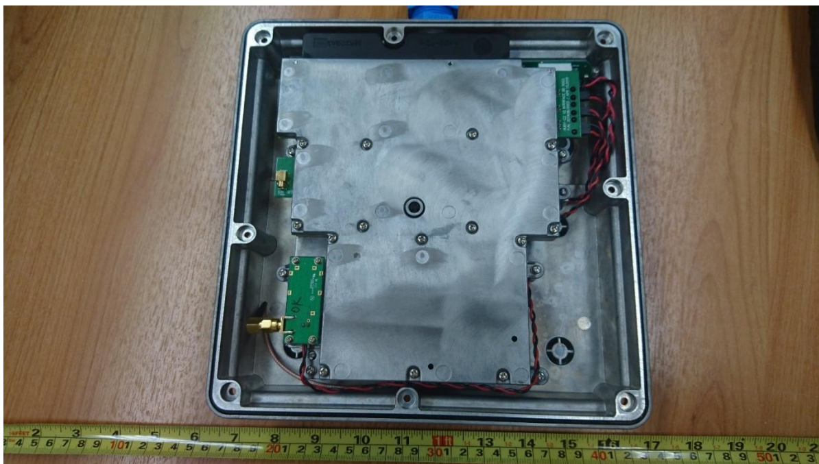
EUT Internal View 1
