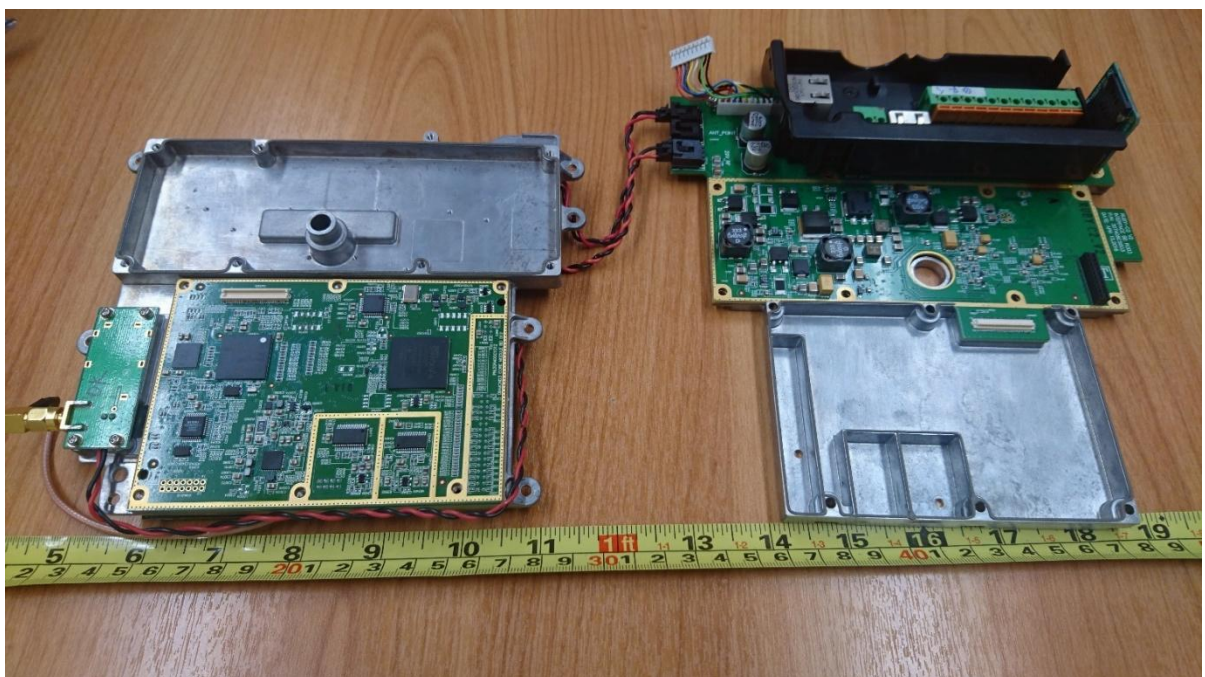
EUT Internal View 4 – Core Module Separated
