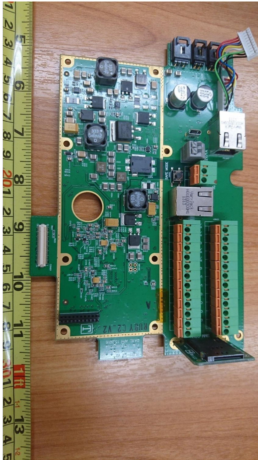
Power Board PCB Component Side
