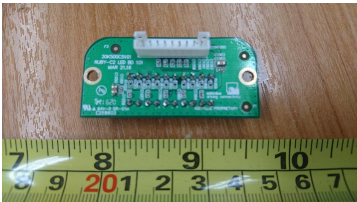
LED PCB Trace Side
