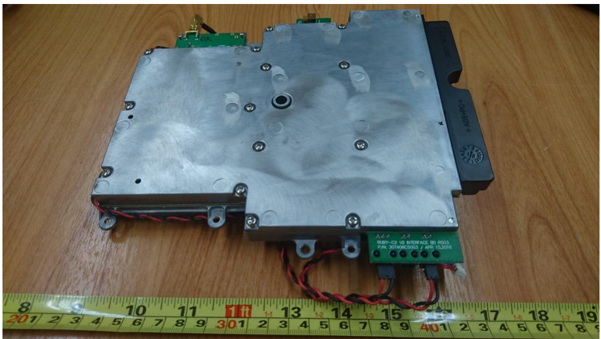
EUT Internal View 3 – Core Module
