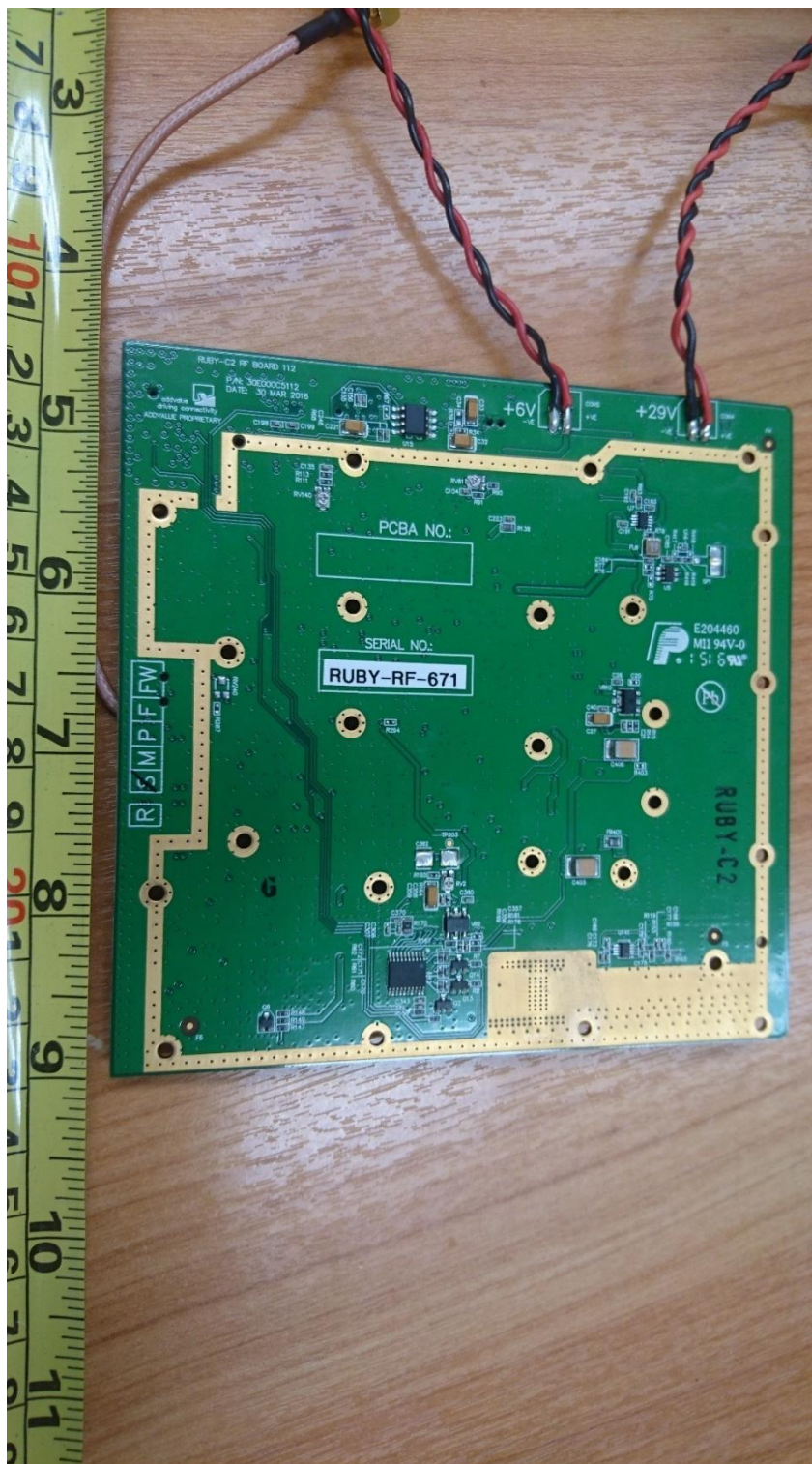
RF PCB Trace Side
