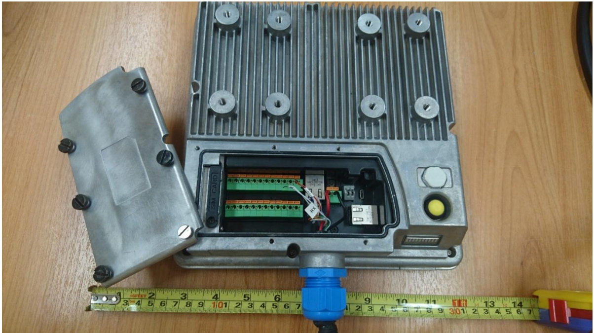
EUT Bottom Internal View 5
