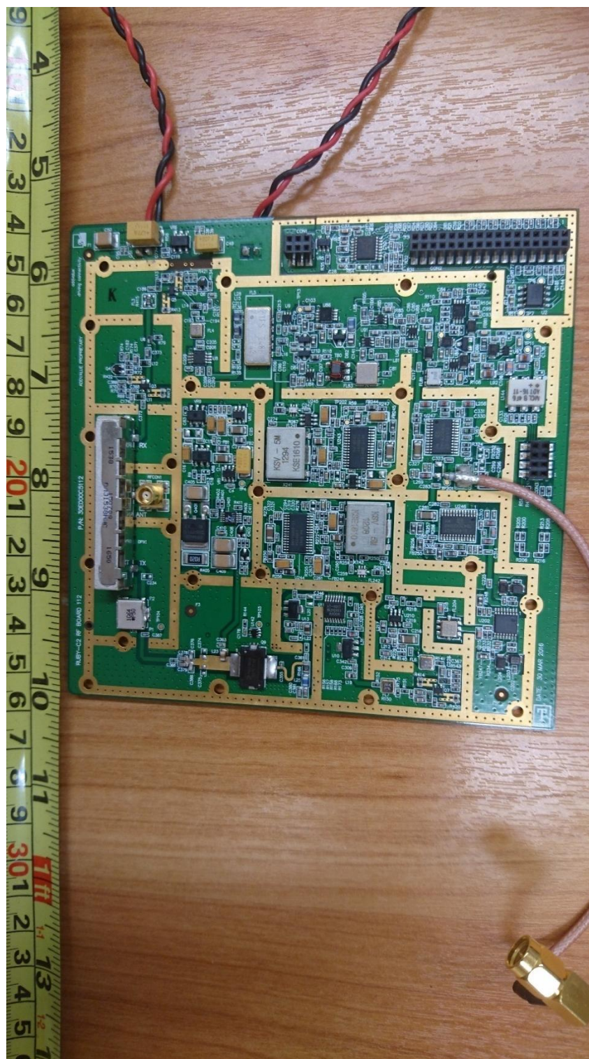
RF PCB Component Side
