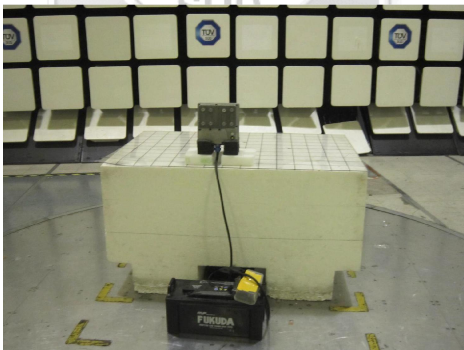
Radiated Spurious Emissions Test Setup (Rear View)
