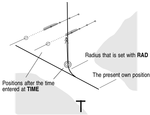
Check by variation of the TIME input
