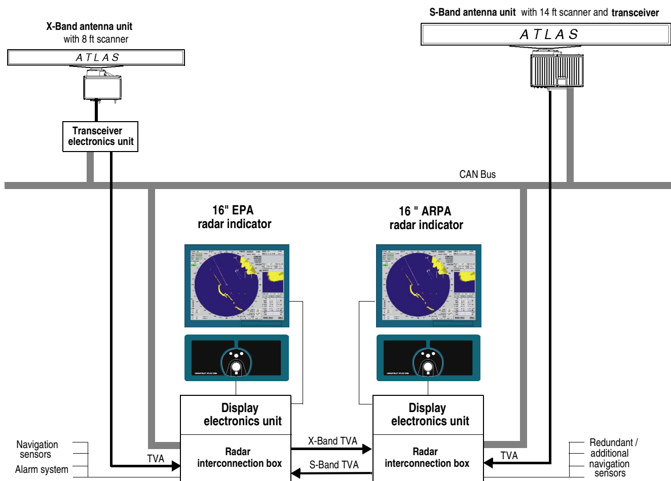
A typical dual installation (IMO pair)
