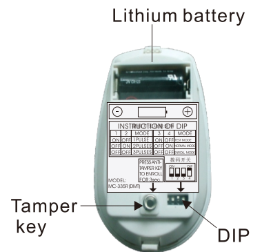
Fig.2. Internal Structure
