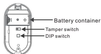
Fig.2 Internal Structure
