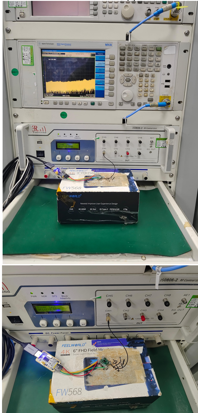
RF Conducted test setup photos
