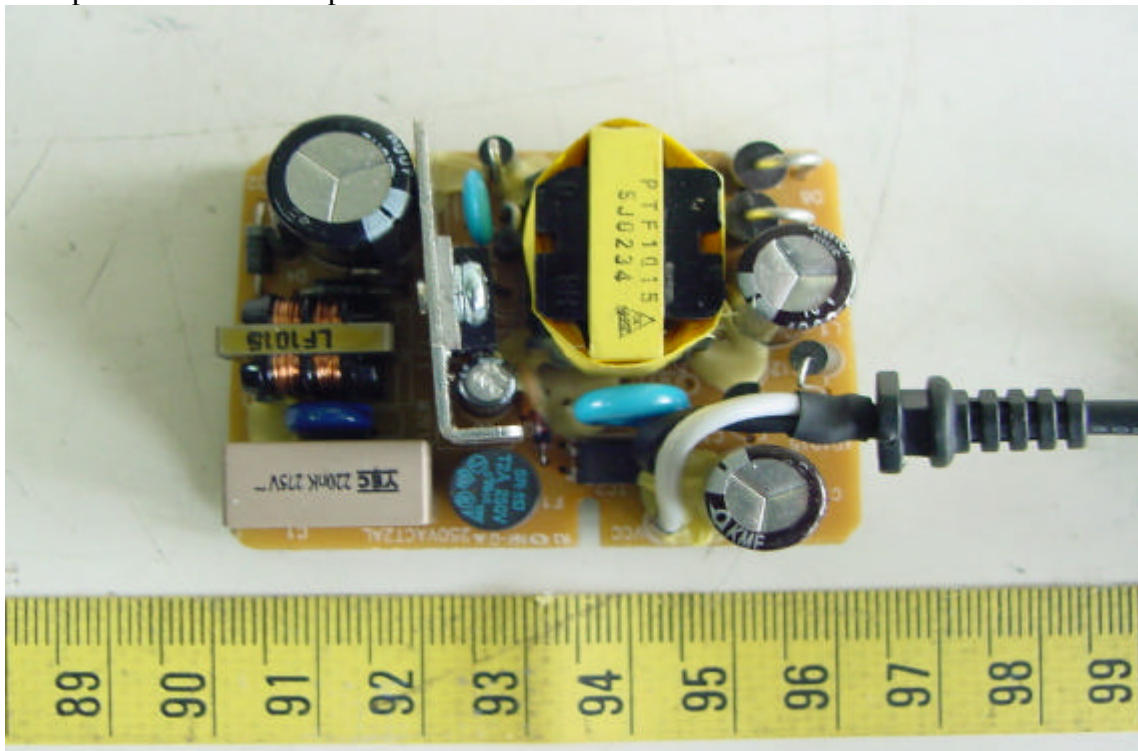
Component View of Adapter
