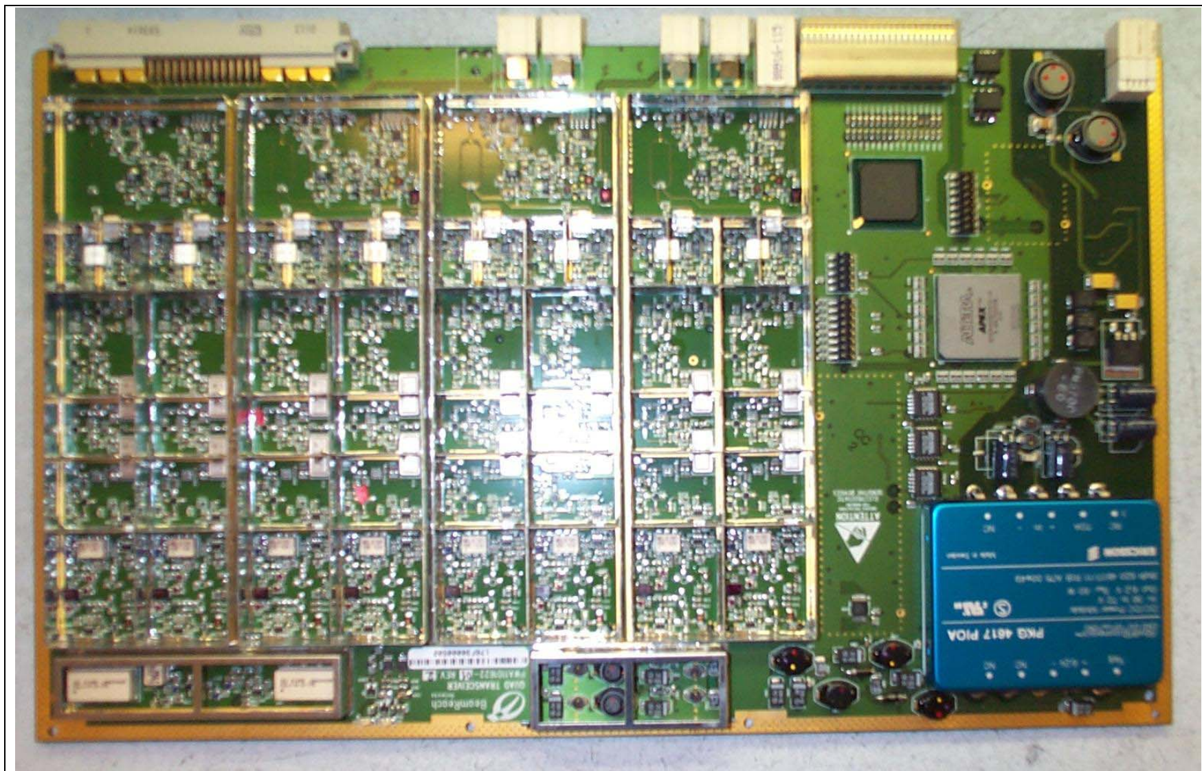
Figure 2. Quad Transceiver Module with shields removed.
