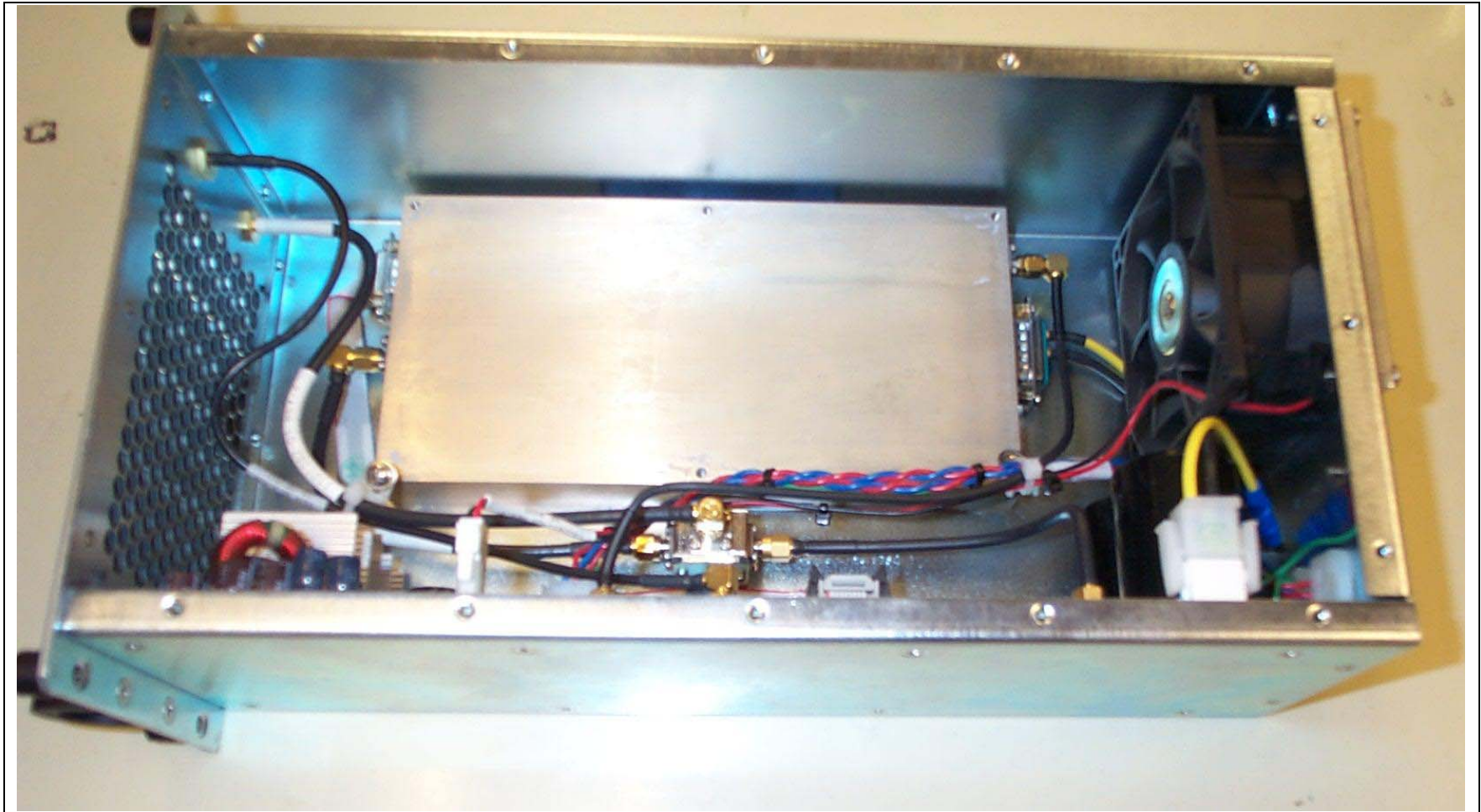
Figure 4. Power Module with power amp heat sink removed, right oblique view.
