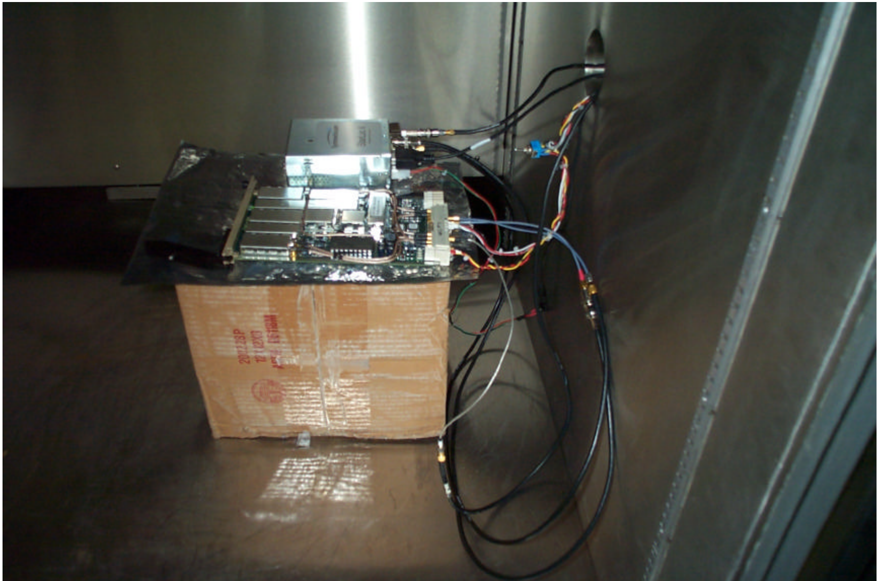
Figure 3. Frequency Stability Test Set-up – close-up of DUT
