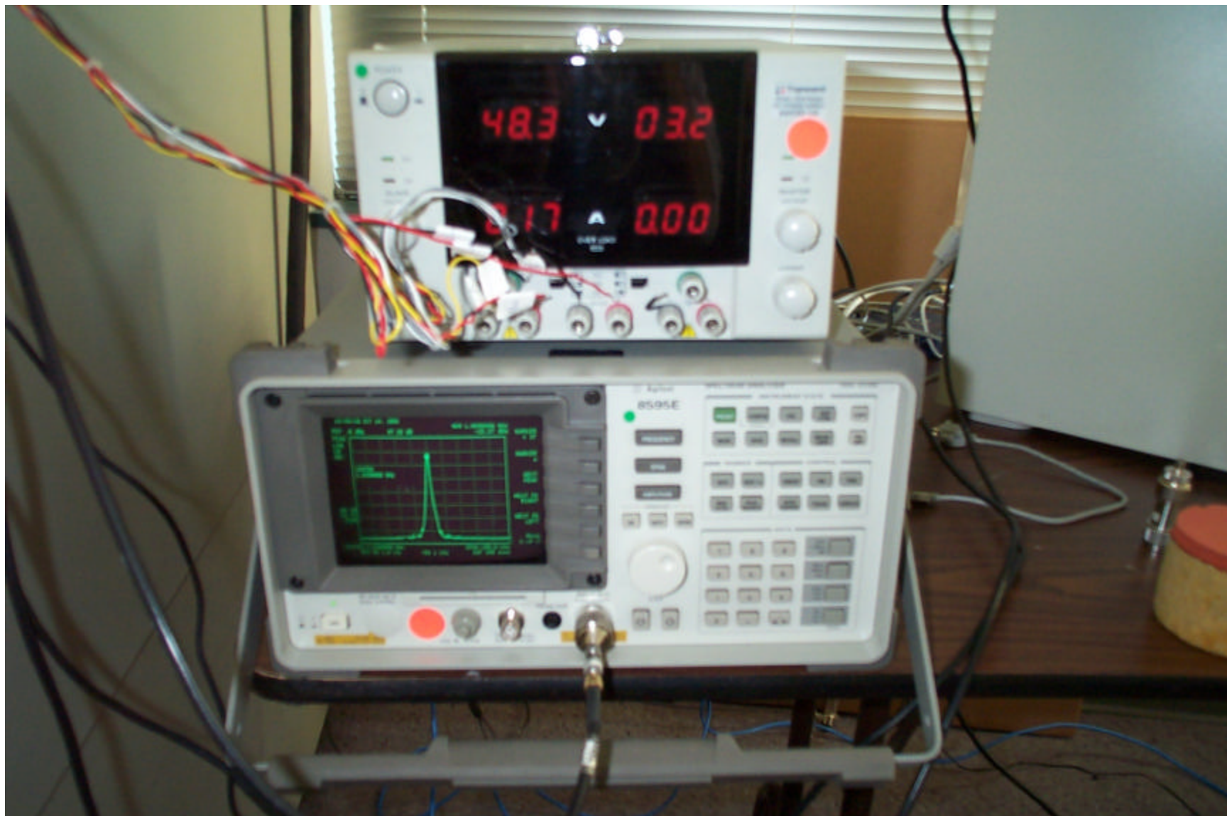
Figure 4. Frequency Stability Test Set-up – close-up of Test Equipment
