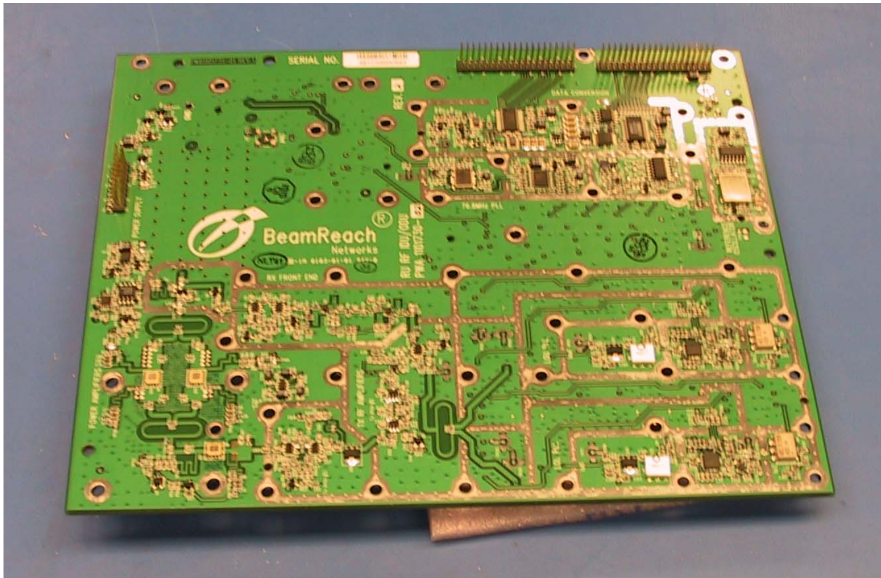
Figure 4. BRU-150 RF PWA, top view, no shields.
