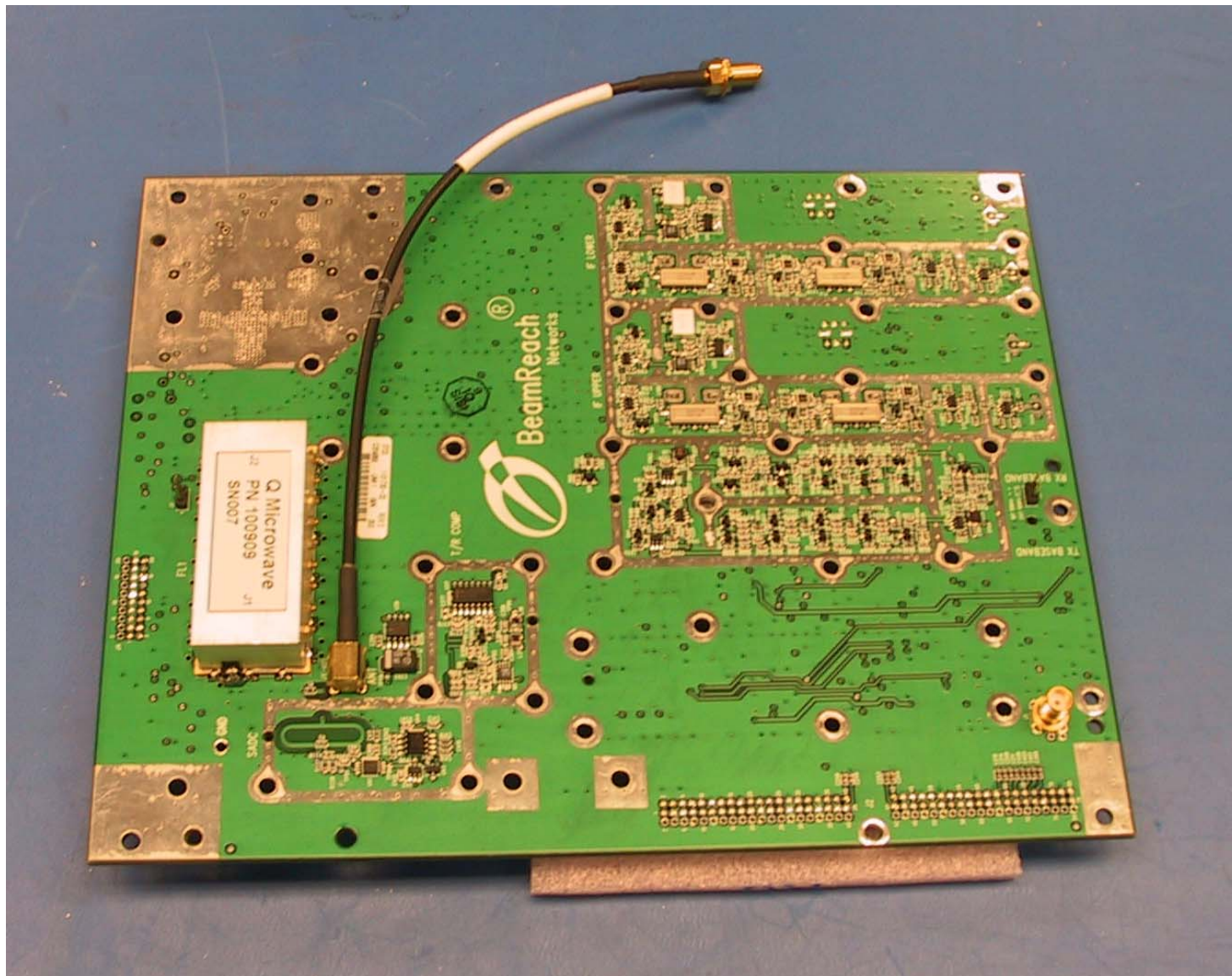
Figure 5. BRU-150 RF PWA, Bottom View, No Shields.
