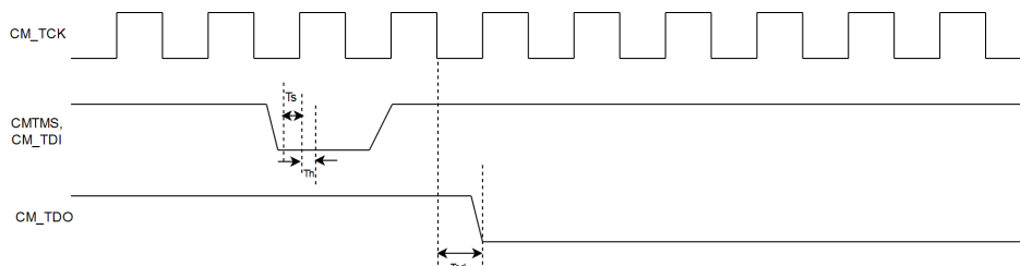
Figure 7.26. Interface Timing Diagram for Cortex-M4 JTAG
