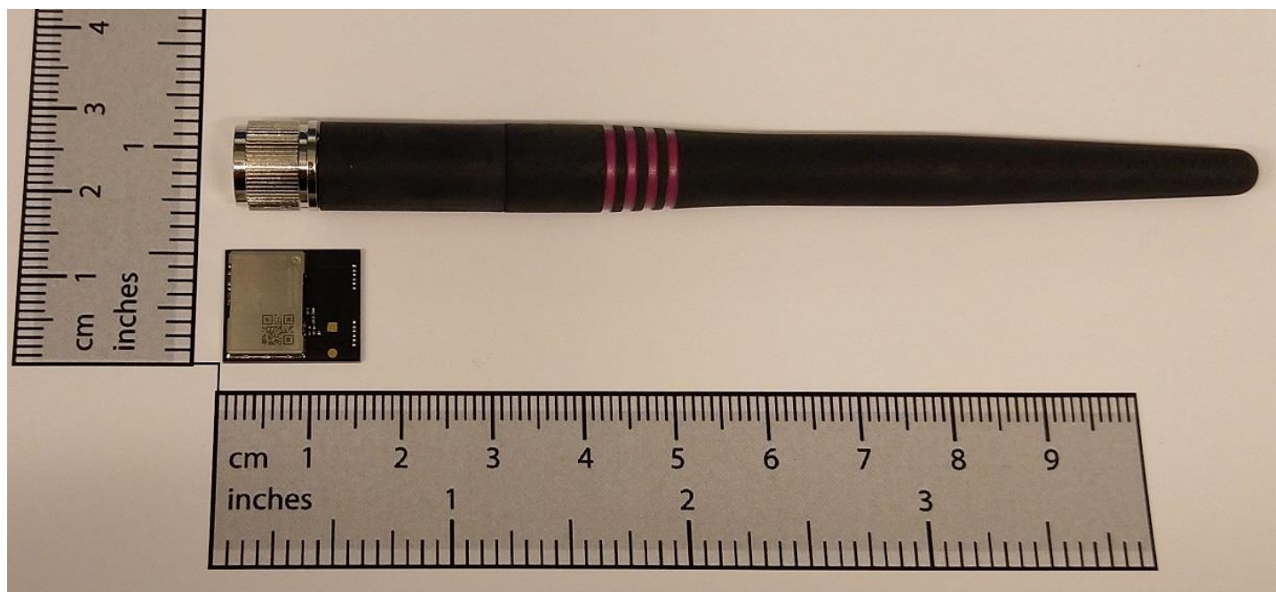
Figure 1: Horizontal Full View of the Reference External Antenna, next to the MGM240P32N Module – Antenna is the ANT-2.4-CW-CT-RPS by Linx Technologies Inc.
