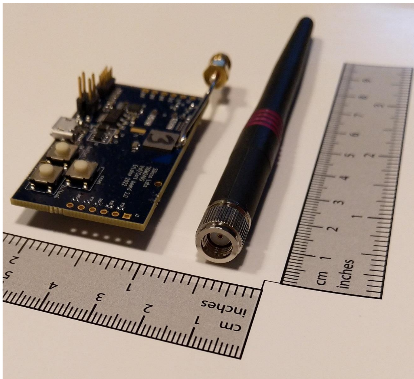
Figure 2 Detail of the External Antenna's RP-SMA Connector. Antenna is the ANT-2.4-CW-CT-RPS by Linx Technologies Inc.
