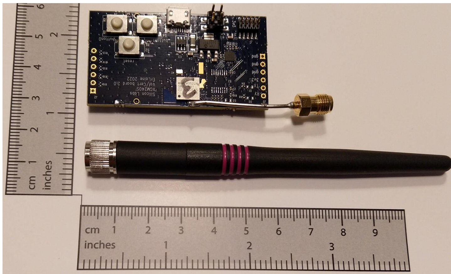
Figure 1 Horizontal Full View of the Reference External Dipole Antenna, next to the Certification Board Carrying the MGM240S22A Module.
