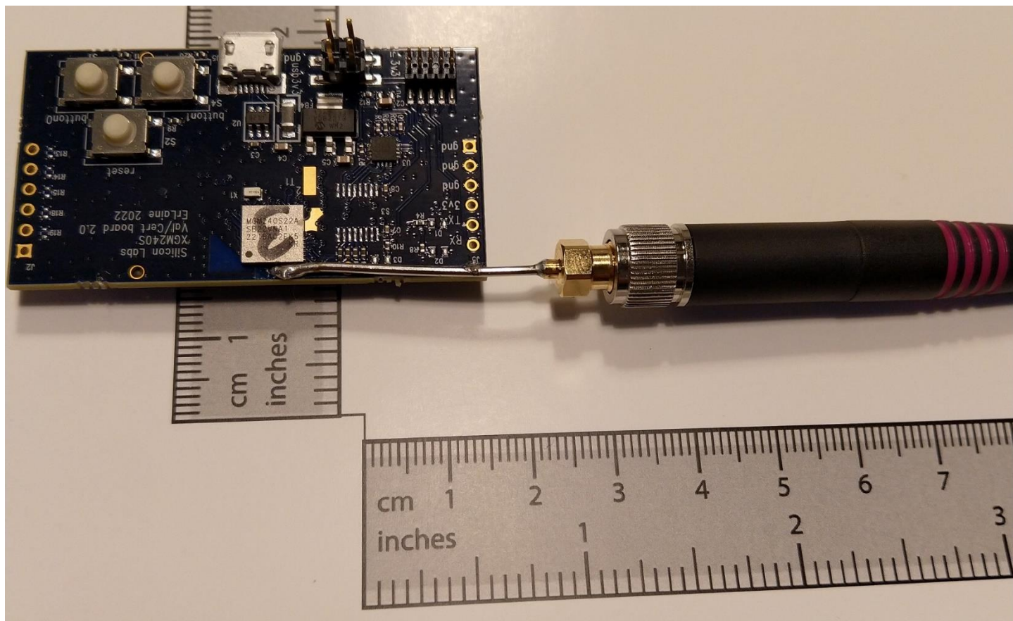
Figure 3 Detail of the External Antenna Connected to the module's RF Pin using a Semi-rigid Coaxial Pigtail Cable
