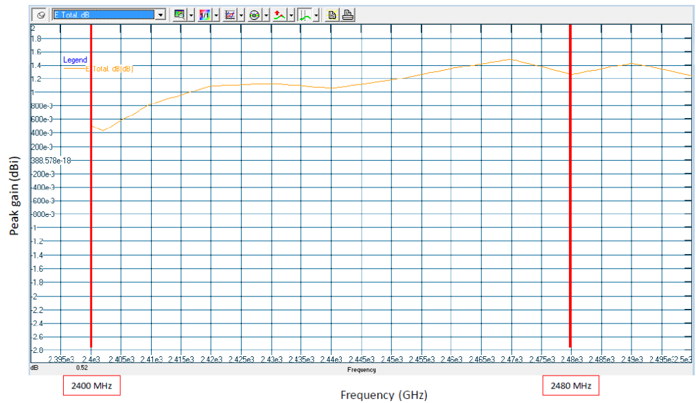
Figure 2: Integral Antenna Gain
