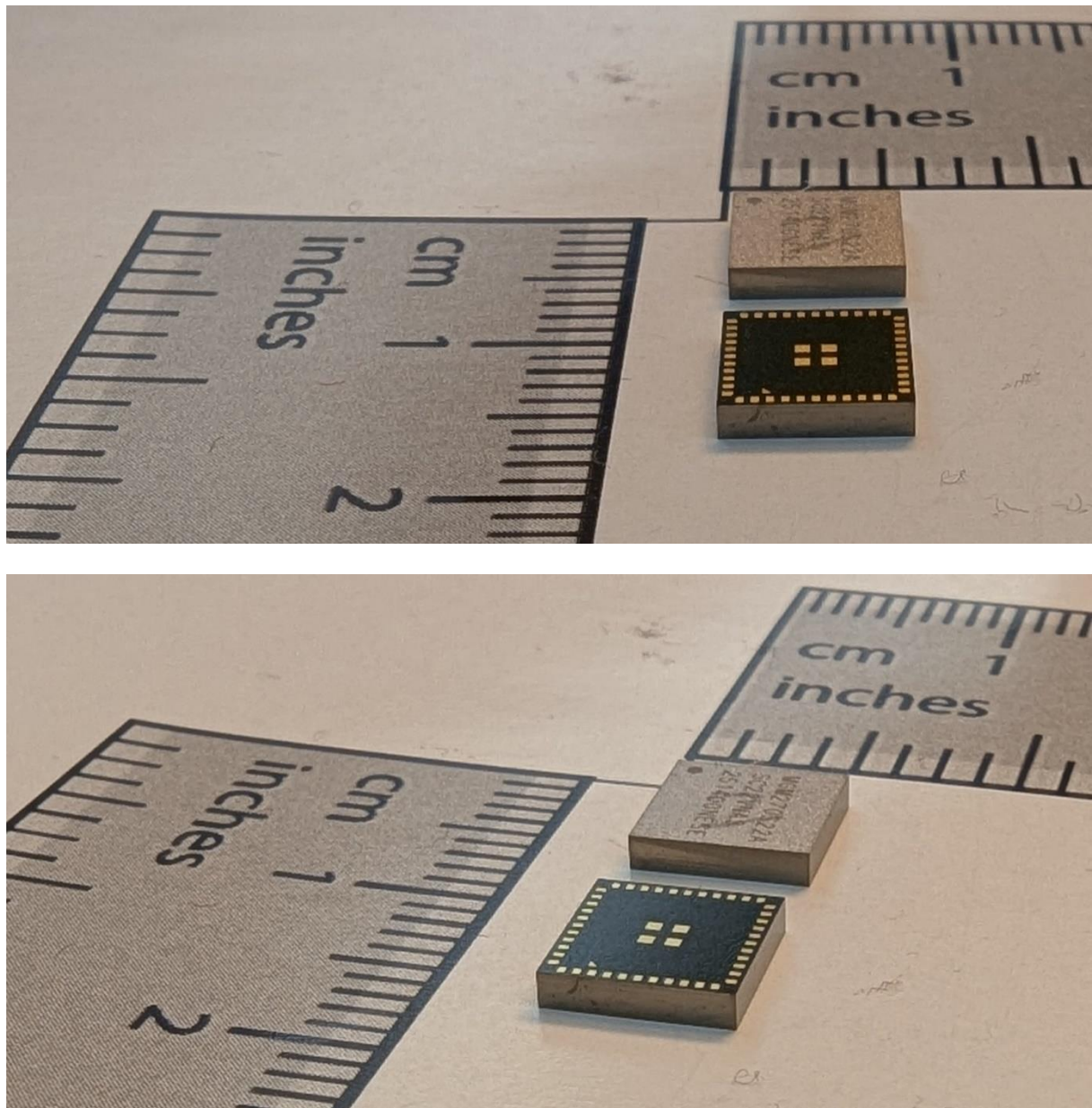
Figure 3: External Side Views of the MGM270S22A Module (Set 2)
