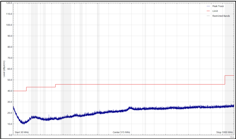
Figure 52- Bottom_2402 MHz, LE500k - 30 MHz to 1 GHz, Vertical (Peak) Y- Orientation
