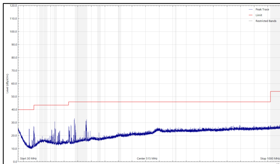
Figure 40- Bottom_ LE500k - 2402 MHz, 30 MHz to 1 GHz, Vertical (Peak) X- Orientation
