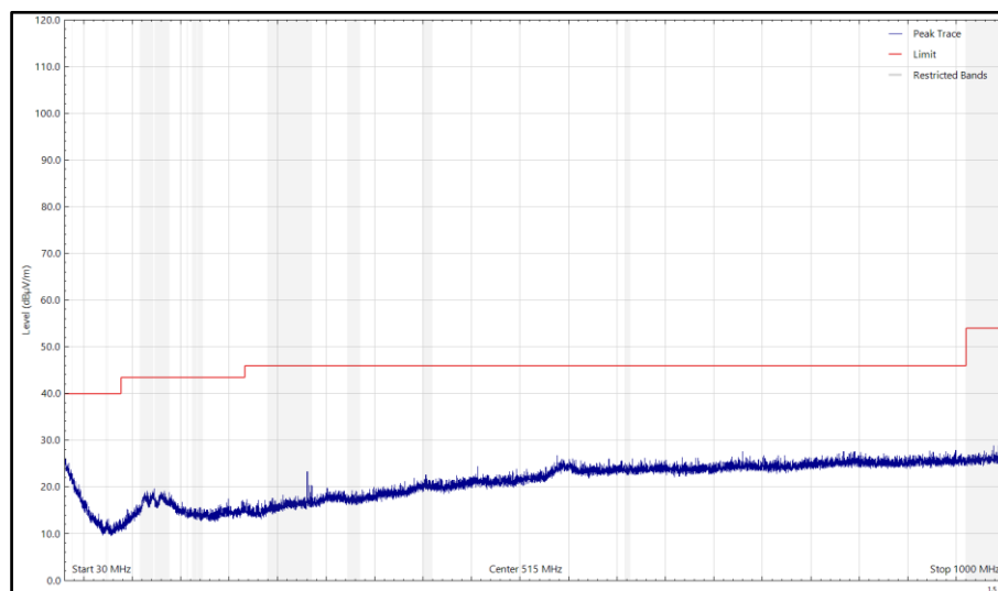
Figure 38- Bottom_LE500k - 2402 MHz, 30 MHz to 1 GHz, Horizontal (Peak) X- Orientation
