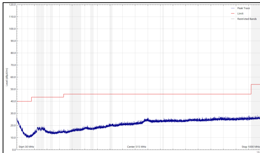
Figure 58- TOP_ 2480 MHz, LE500k - 30 MHz to 1 GHz, Horizontal (Peak) Y-Orientation
