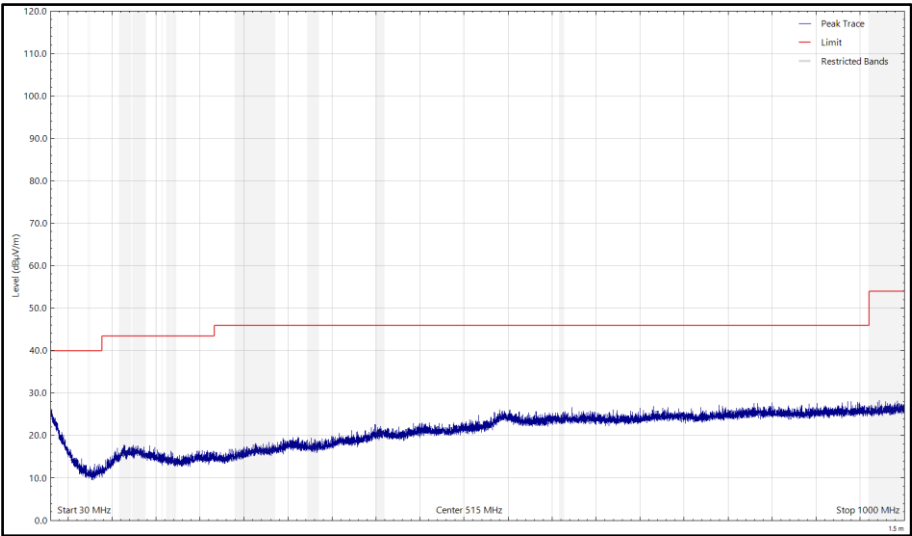
Figure 64- Bottom_2402 MHz, LE500k - 30 MHz to 1 GHz, Vertical (Peak) Z- Orientation
