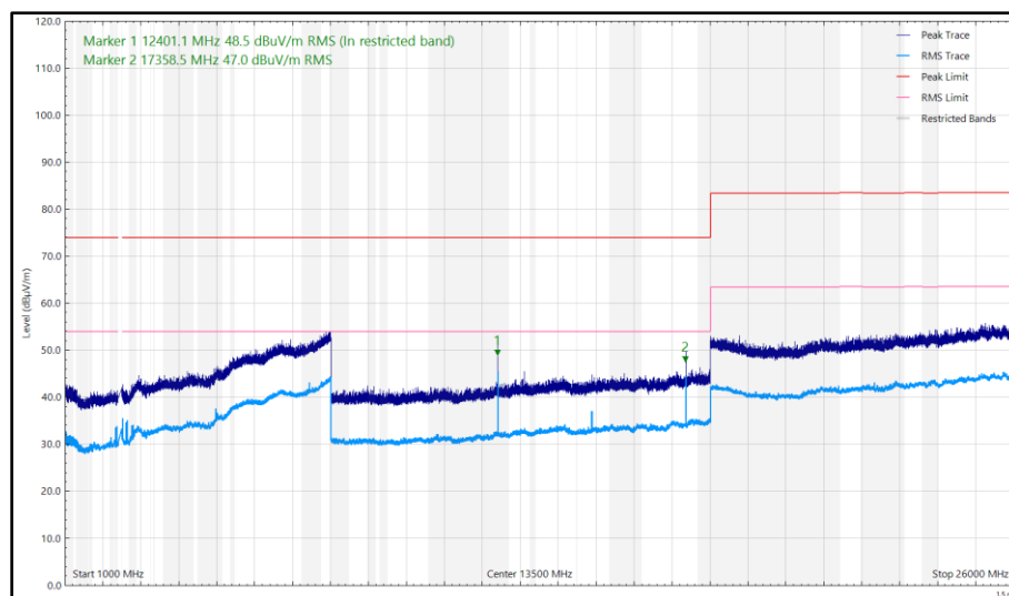
Figure 71- TOP_2480 MHz, LE500k - 1 GHz to 26 GHz, Horizontal (Peak) Z-Orientation
