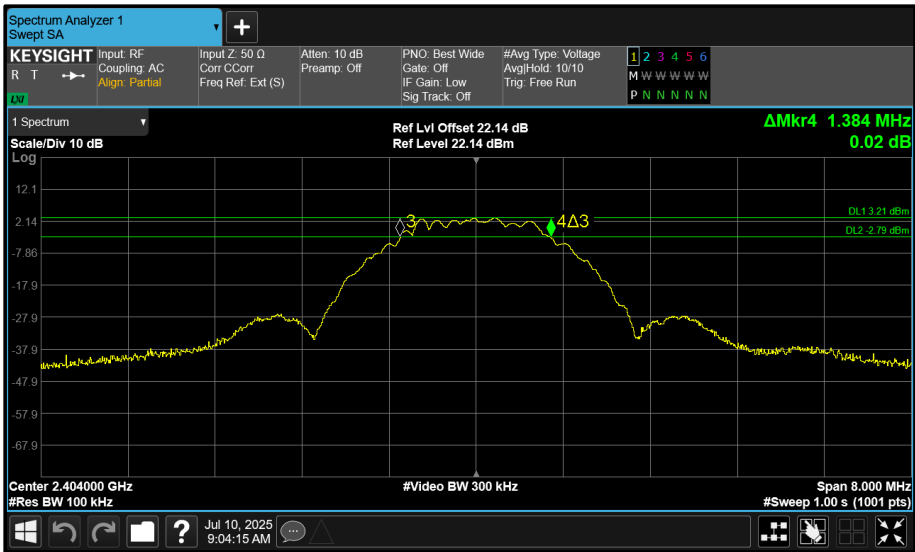
Figure 8 - 2404 MHz (CH37) 6 dB Bandwidth
