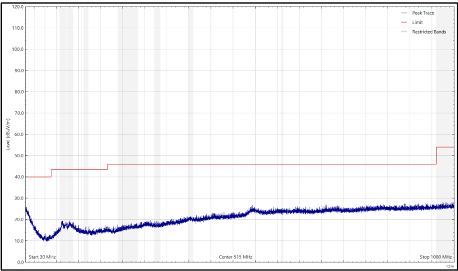
Figure 54- Mid_BLE_2402 MHz, LE500k - 30 MHz to 1 GHz, Horizontal (Peak) Y- Orientation
