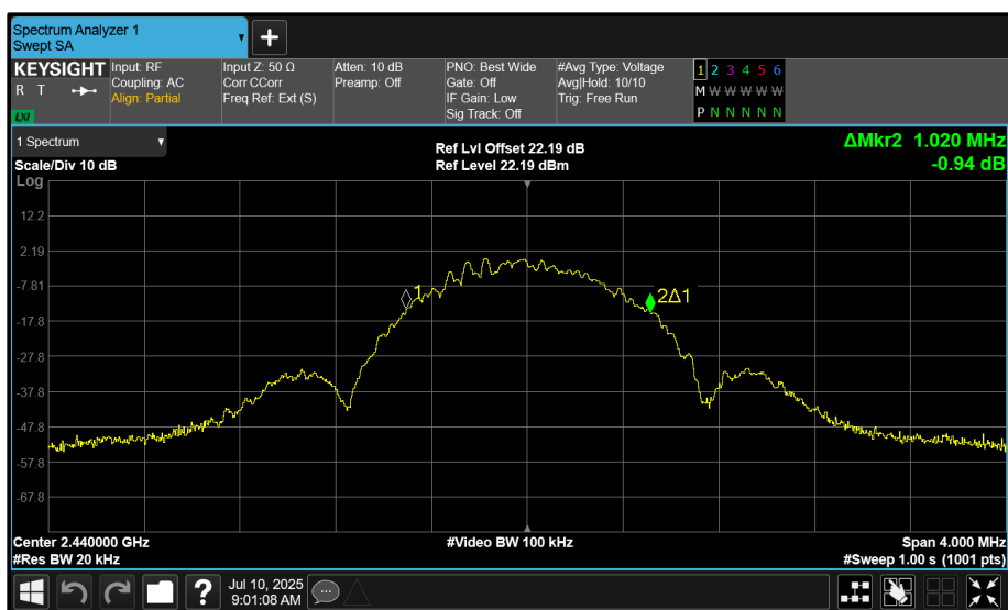
Figure 3 - 2440 MHz (CH 17) 99% Bandwidth
