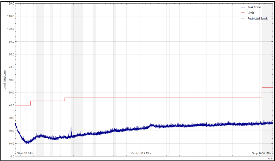
Figure 48- Top_2480 MHz, LE500k - 30 MHz to 1 GHz, Vertical (Peak) X-Orientation
