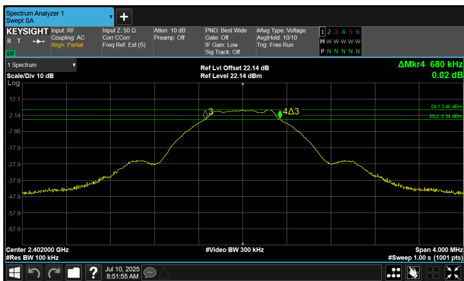
Figure 2 - 2402 MHz (CH37) 6 dB Bandwidth
