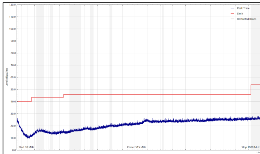
Figure 44- Mid_ 2440 MHz, LE500k - 30 MHz to 1 GHz, Vertical (Peak) X-Orientation
