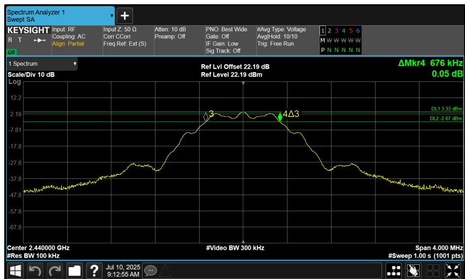
Figure 22 - 2440 MHz (CH17) 6 dB Bandwidth
