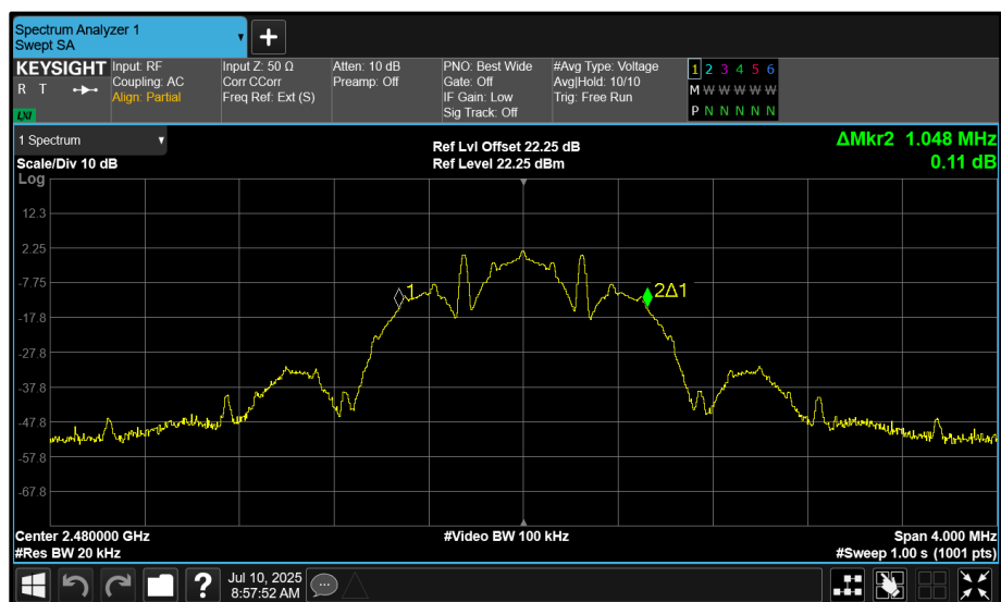
Figure 23 - 2480 MHz (CH39) 99% Bandwidth
