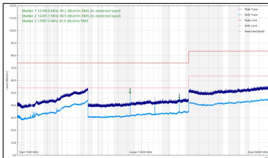
Figure 67- Mid_2440 MHz, LE500k - 1 GHz to 26 GHz, Horizontal (Peak) Z- Orientation
