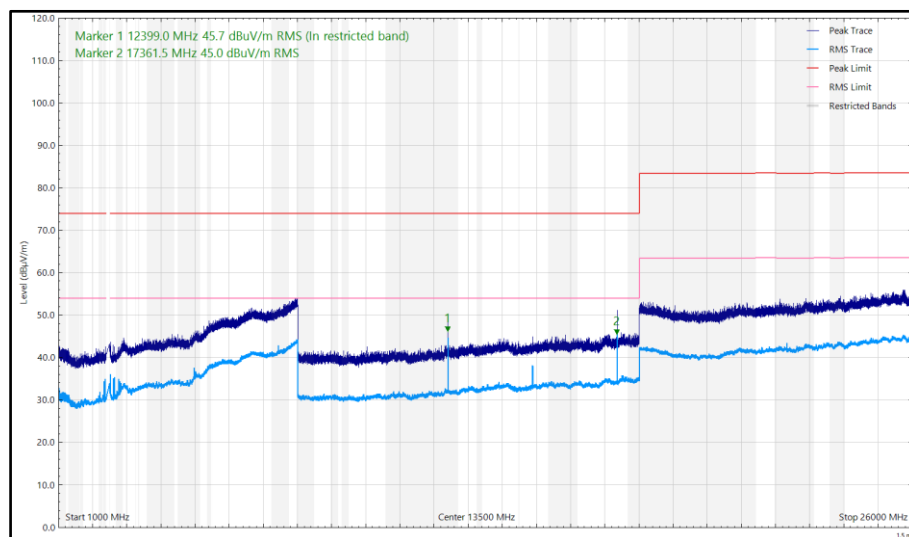
Figure 61- TOP_2480 MHz, LE500k - 1 GHz to 26 GHz, Vertical (Peak) Y-Orientation
