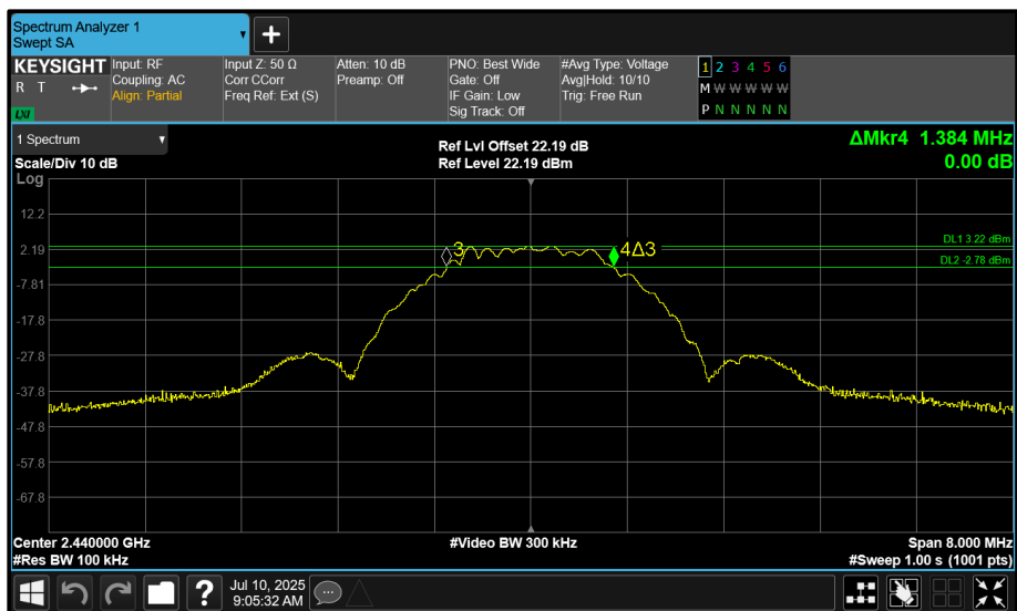
Figure 10 - 2440 MHz (CH17) 6 dB Bandwidth
