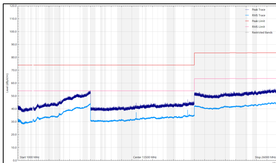
Figure 59- TOP_ 2480 MHz, LE500k - 1 GHz to 26 GHz, Horizontal (Peak) Y-Orientation
