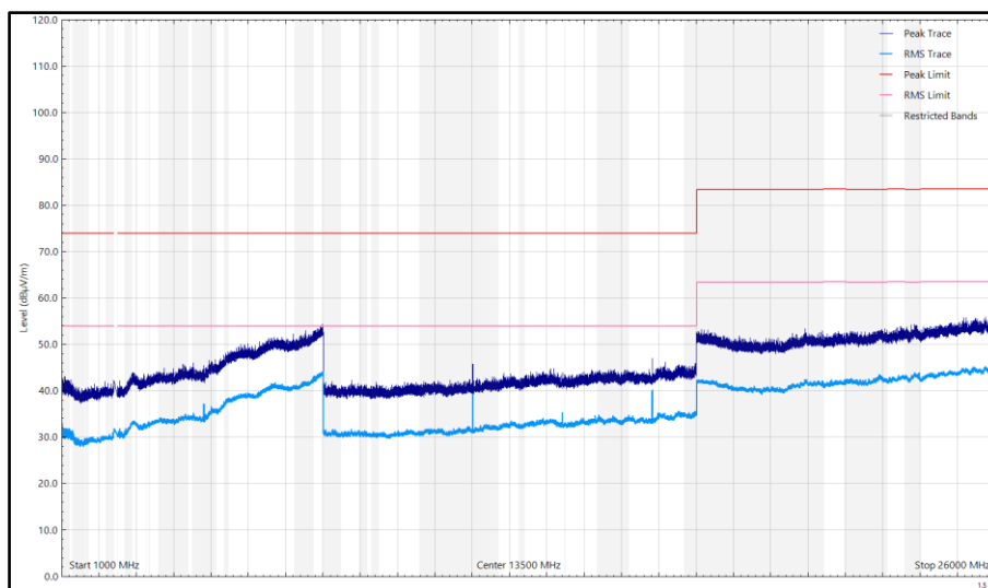
Figure 51- Bottom_ 2402 MHz, LE500k - 1 GHz to 26 GHz, Horizontal (Peak) Y- Orientation
