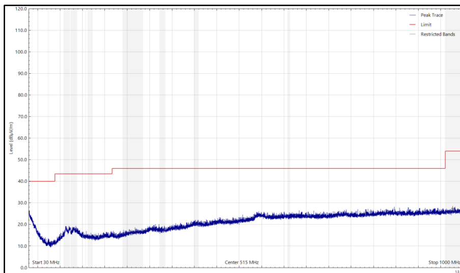
Figure 50- Bottom_ 2402 MHz, LE500k - 30 MHz to 1 GHz, Horizontal (Peak) Y- Orientation
