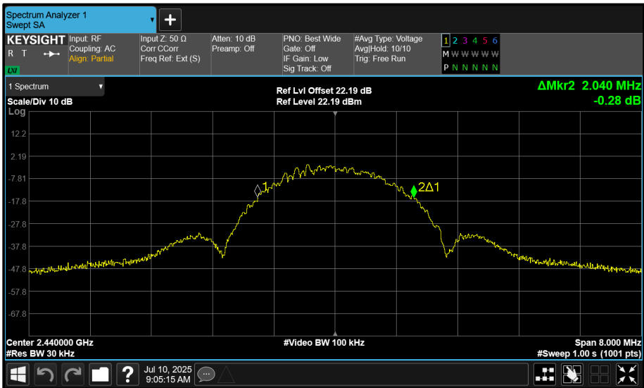
Figure 9 - 2440 MHz (CH39) 99% Bandwidth
