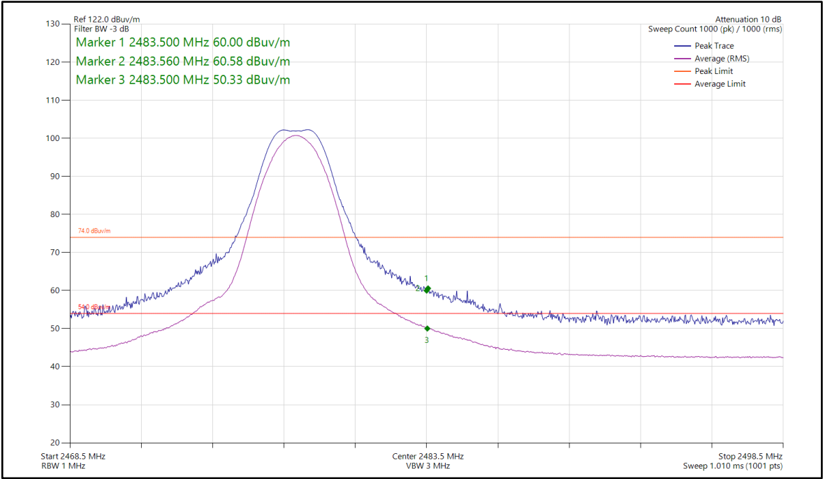
Figure 32 - TOP_BLE_1M_LE2M, 2478 MHz, Band Edge Frequency 2483.5 MHz
