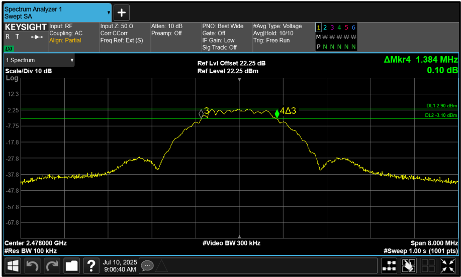
Figure 12 - 2478 MHz (CH39) 6 dB Bandwidth
