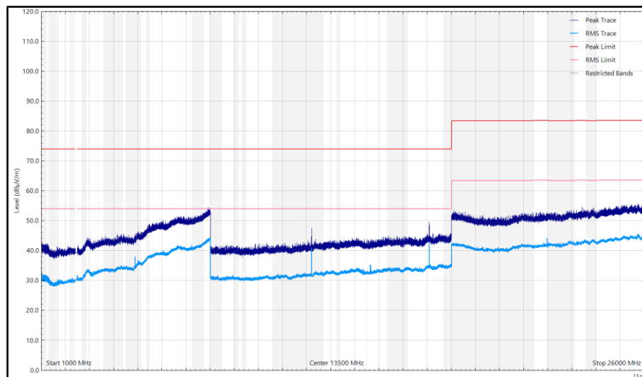
Figure 69- Mid_2440 MHz, LE500k - 1 GHz to 26 GHz, Vertical (Peak) Z- Orientation
