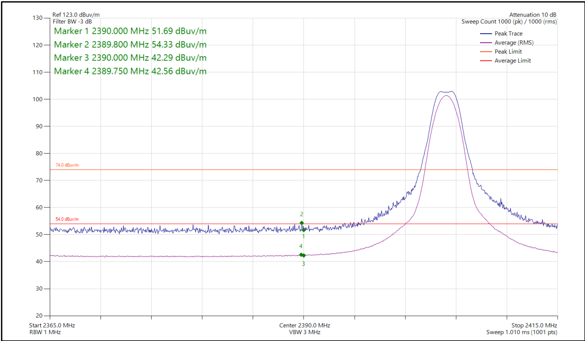
Figure 31 - BOT_BLE_1M_LE2M, 2404 MHz, Band Edge Frequency 2390 MHz
