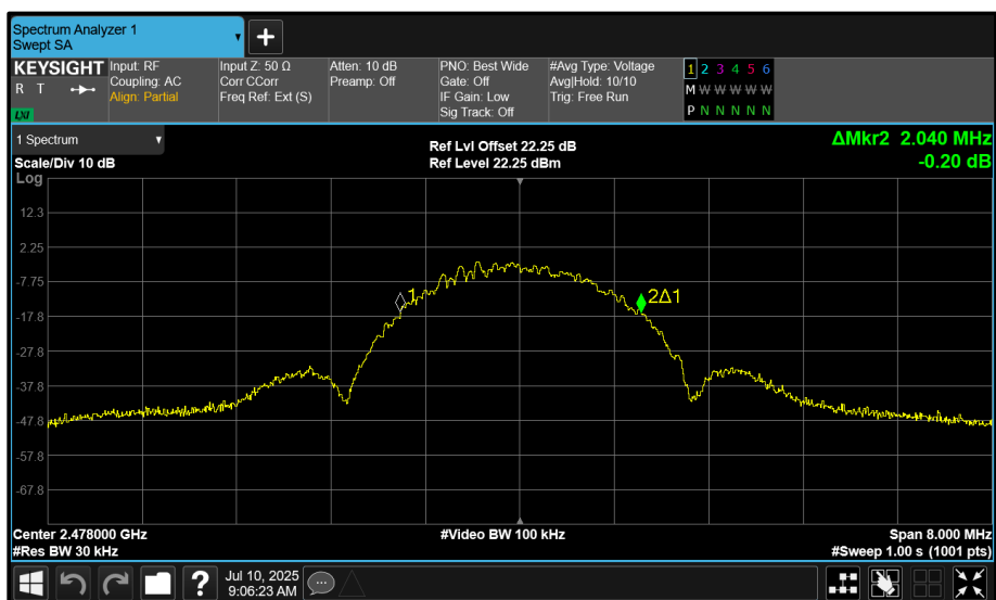
Figure 11 - 2478 MHz (CH39) 99% Bandwidth
