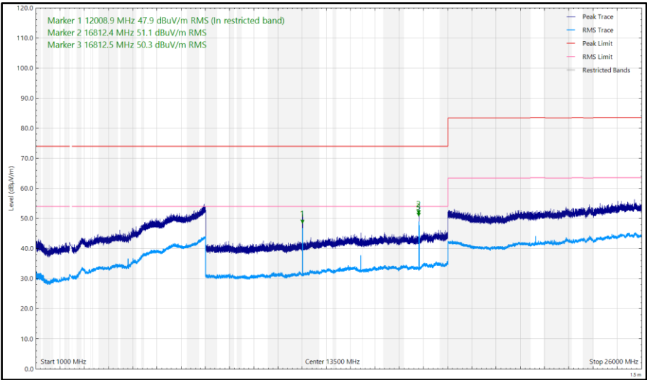
Figure 41- Bottom_ LE500k - 2402 MHz, 1 GHz to 26 GHz, Vertical (Peak) X- Orientation
