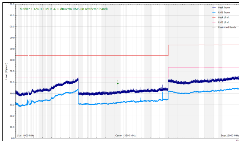
Figure 47- Top_2480 MHz, LE500k - 1 GHz to 26 GHz, Horizontal (Peak) X-Orientation
