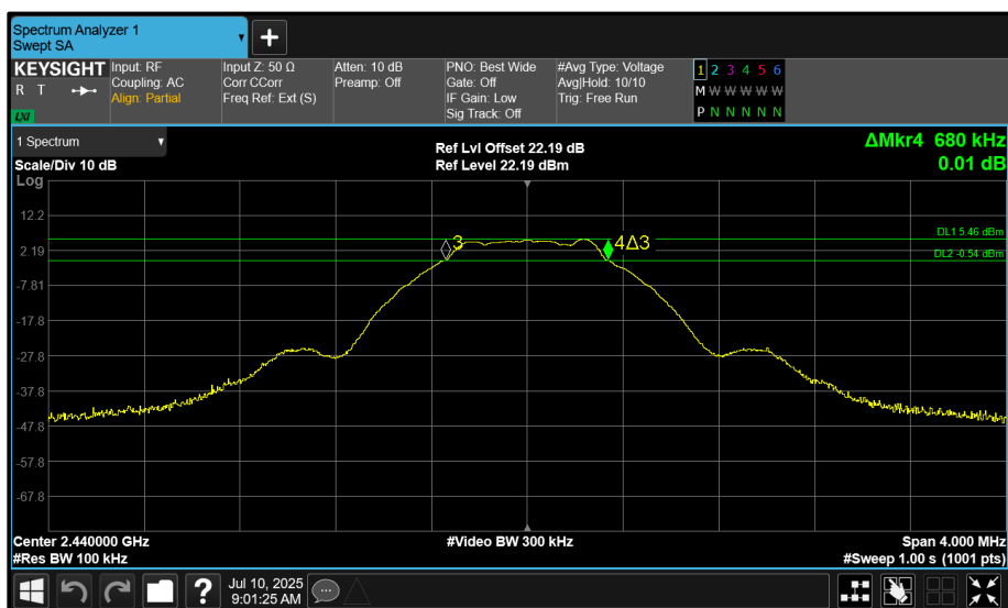
Figure 4 - 2440 MHz (CH17) 6 dB Bandwidth
