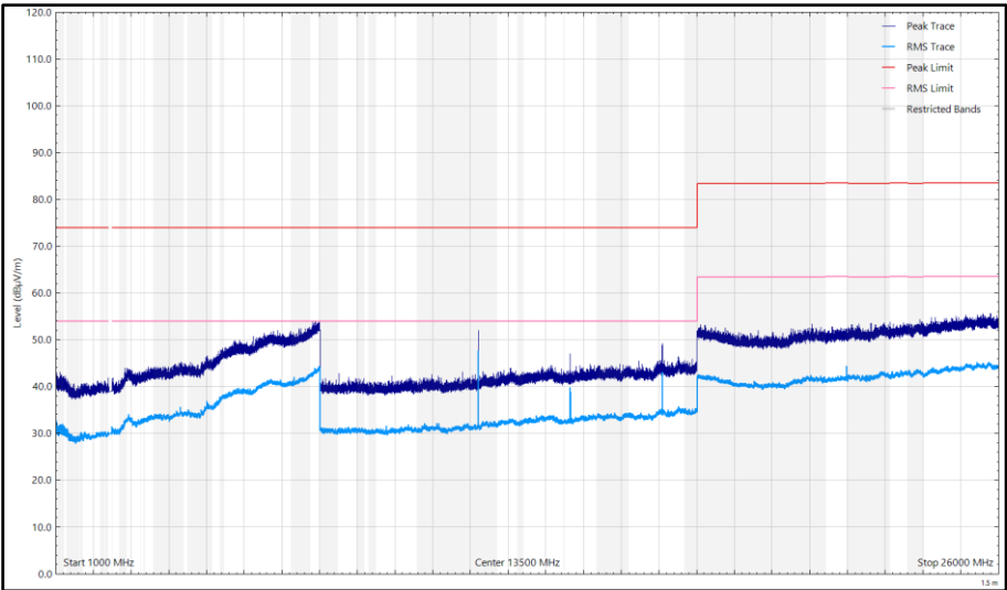
Figure 57- Mid_ 2402 MHz, LE500k - 1 GHz to 26 GHz, Vertical (Peak) Y- Orientation
