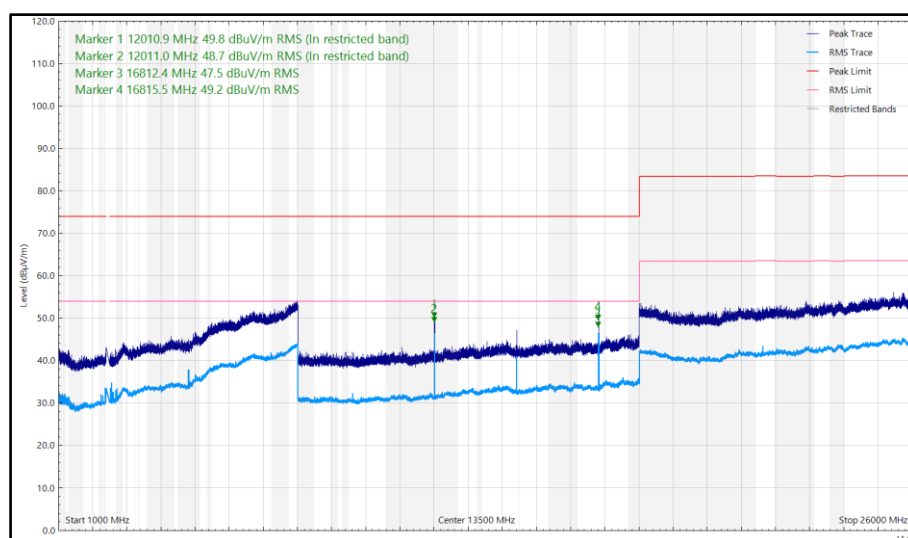
Figure 63- Bottom_2402 MHz, LE500k - 1 GHz to 26 GHz, Horizontal (Peak) Z- Orientation
