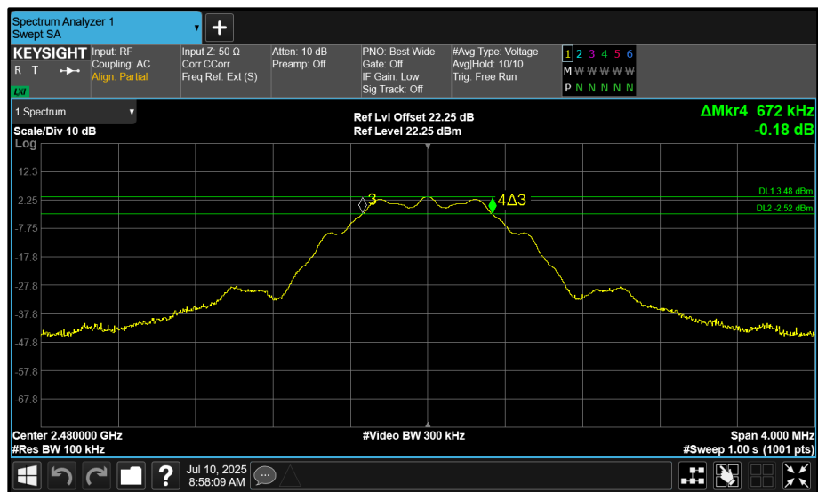
Figure 24 - 2480 MHz (CH39) 6 dB Bandwidth
