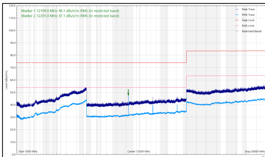
Figure 43- Mid_ 2440 MHz, LE500k - 1 GHz to 26 GHz, Horizontal (Peak) X-Orientation
