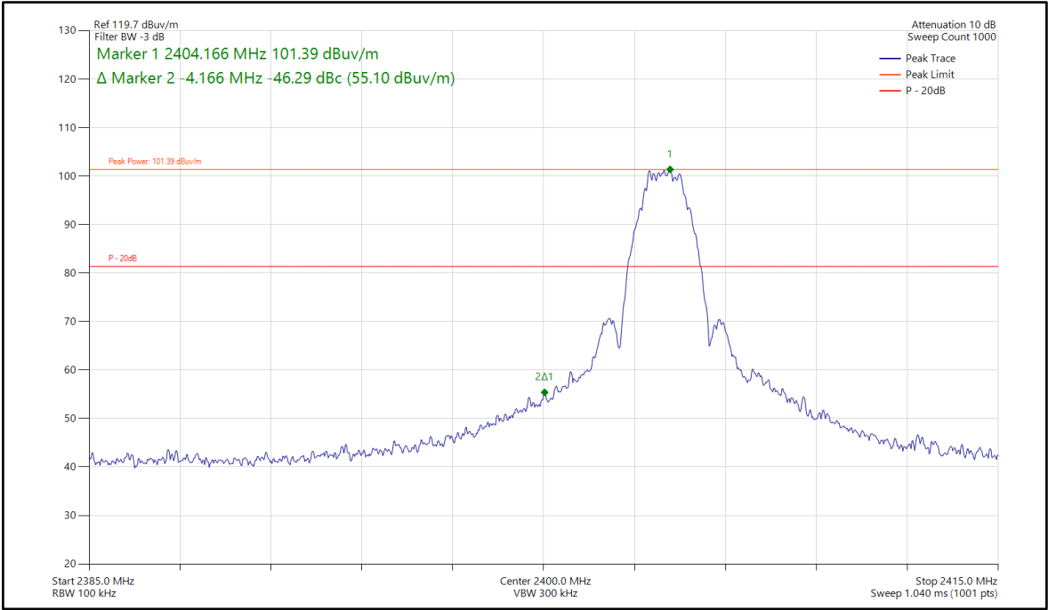
Figure 34 - BOT_BLE_2M_2404 MHz, Band Edge Frequency 2400 MHz
