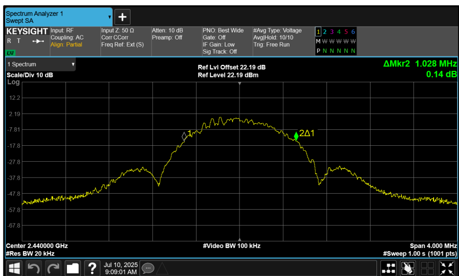
Figure 15 - 2440 MHz (CH17) 99% Bandwidth
