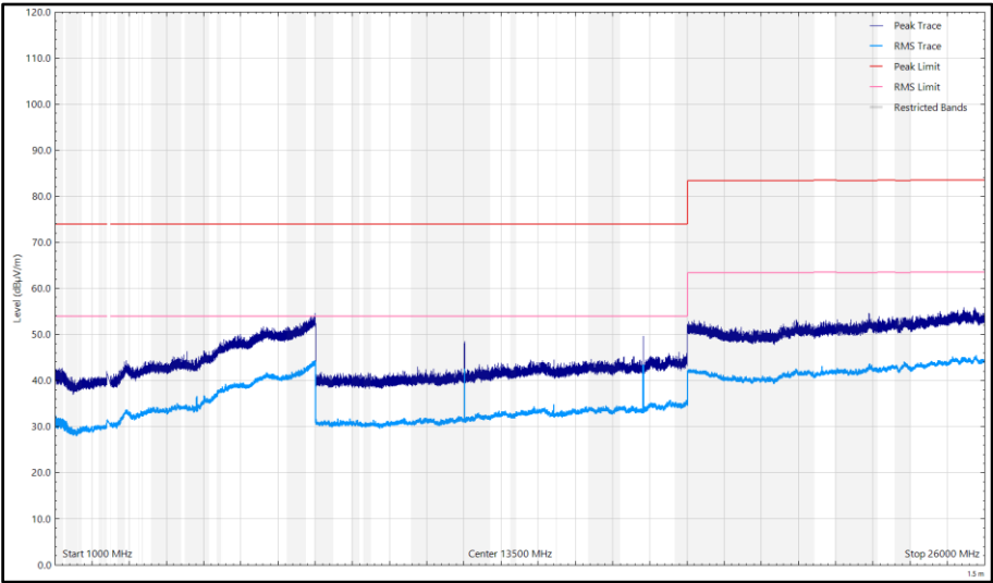
Figure 65- Bottom_2402 MHz, LE500k - 1 GHz to 26 GHz, Vertical (Peak) Z- Orientation
