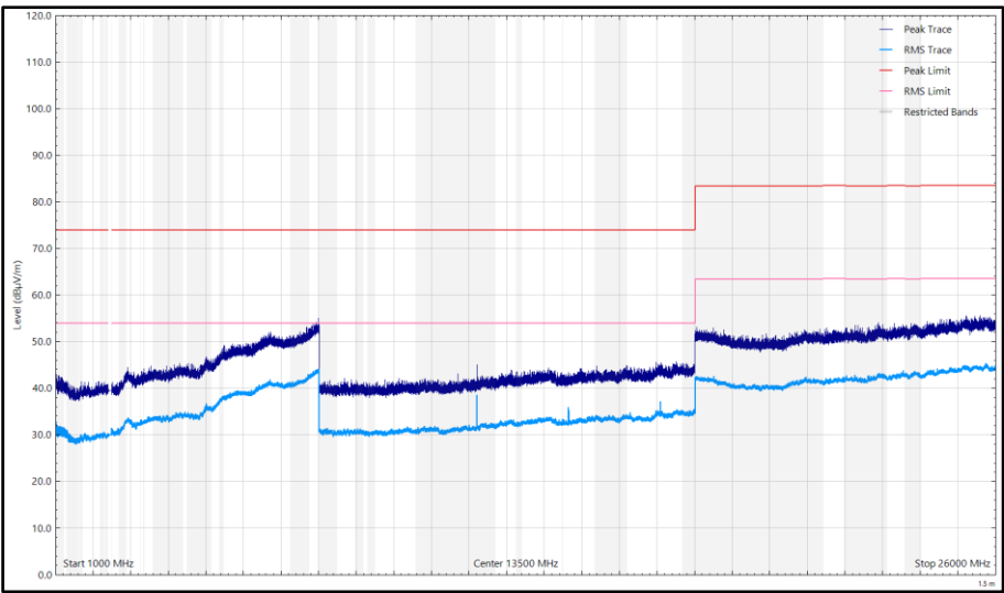
Figure 55- Mid_ 2402 MHz, LE500k - 1 GHz to 26 GHz, Horizontal (Peak) Y- Orientation
