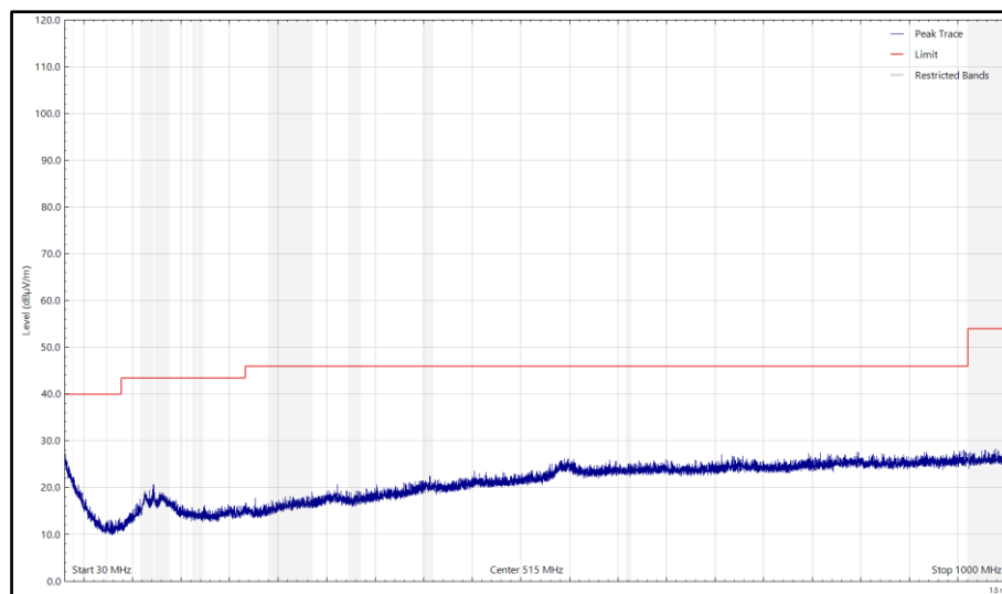
Figure 70- TOP_2480 MHz, LE500k - 30 MHz to 1 GHz, Horizontal (Peak) Z -Orientation
