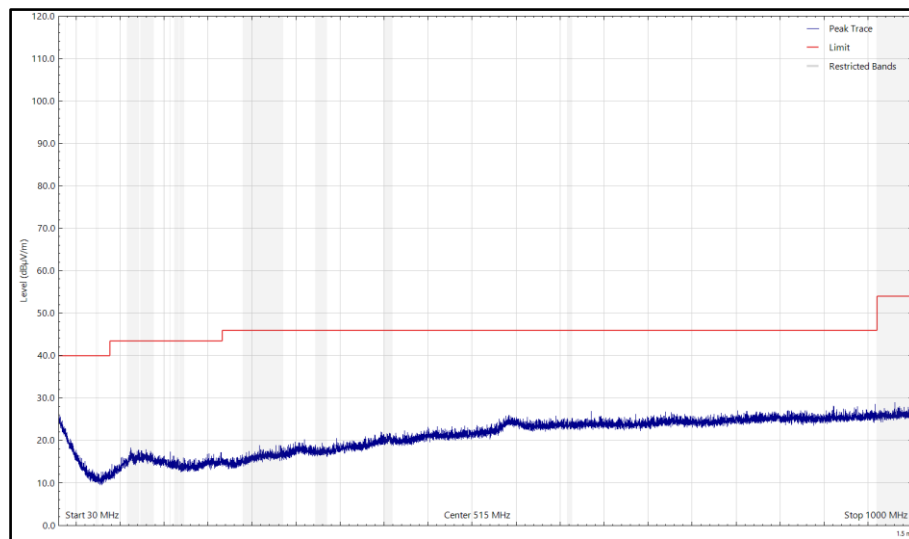
Figure 68- Mid_2440 MHz, LE500k - 30 MHz to 1 GHz, Vertical (Peak) Z- Orientation
