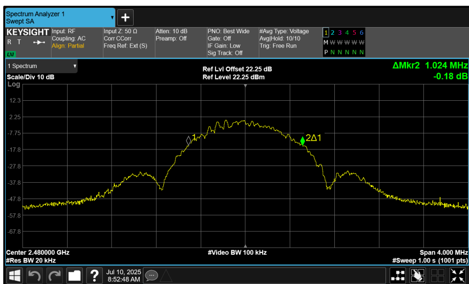
Figure 5 - 2480 MHz (CH39) 99% Bandwidth
