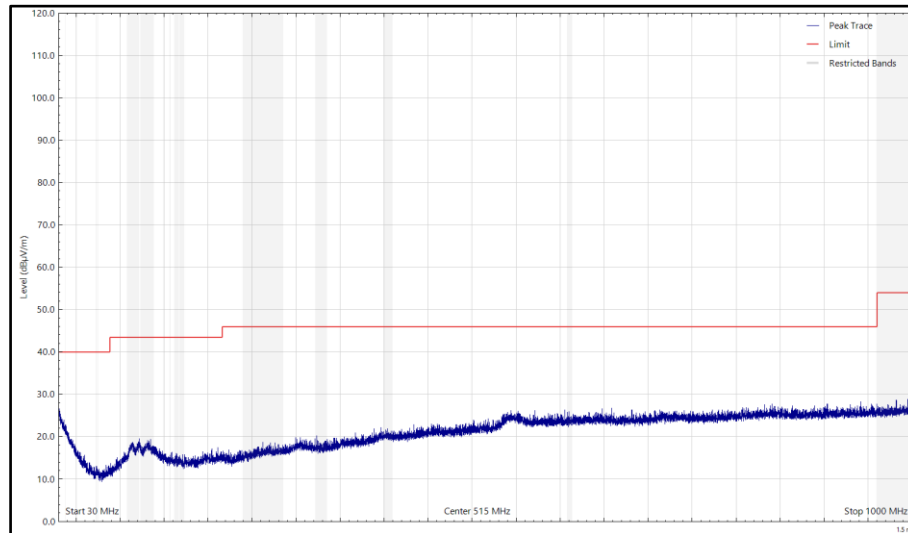
Figure 46- Top_ 2480 MHz, LE500k - 30 MHz to 1 GHz, Horizontal (Peak) X-Orientation
