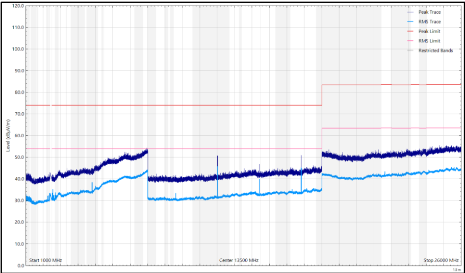
Figure 53- Bottom_2402 MHz, LE500k - 1 GHz to 26 GHz, Vertical (Peak) Y- Orientation
