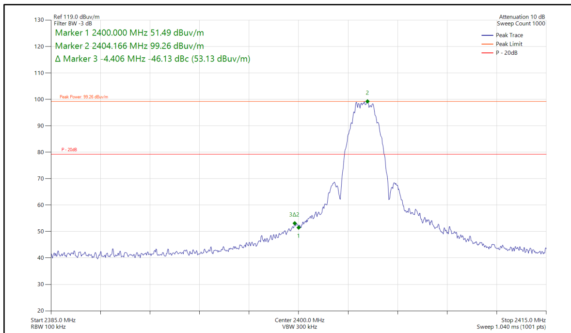
Figure 36 - BOT_BLE_2M_2404 MHz, Band Edge Frequency 2400 MHz
