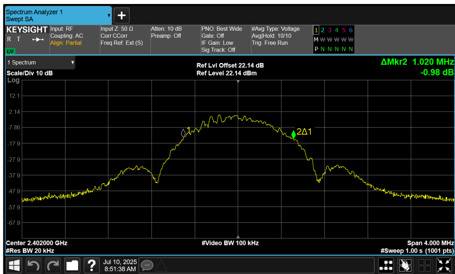
Figure 1 - 2402 MHz (CH37) 99% Bandwidth
