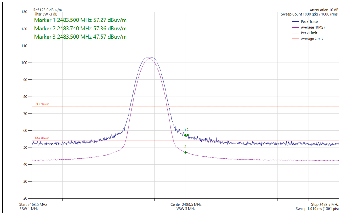
Figure 26 - TOP_BLE_1M_2480 MHz, Band Edge Frequency 2483.5 MHz
