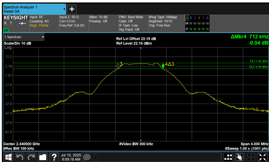
Figure 16 - 2440 MHz (CH17) 6 dB Bandwidth
