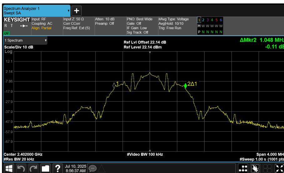
Figure 19 - 2402 MHz (CH37) 99% Bandwidth
