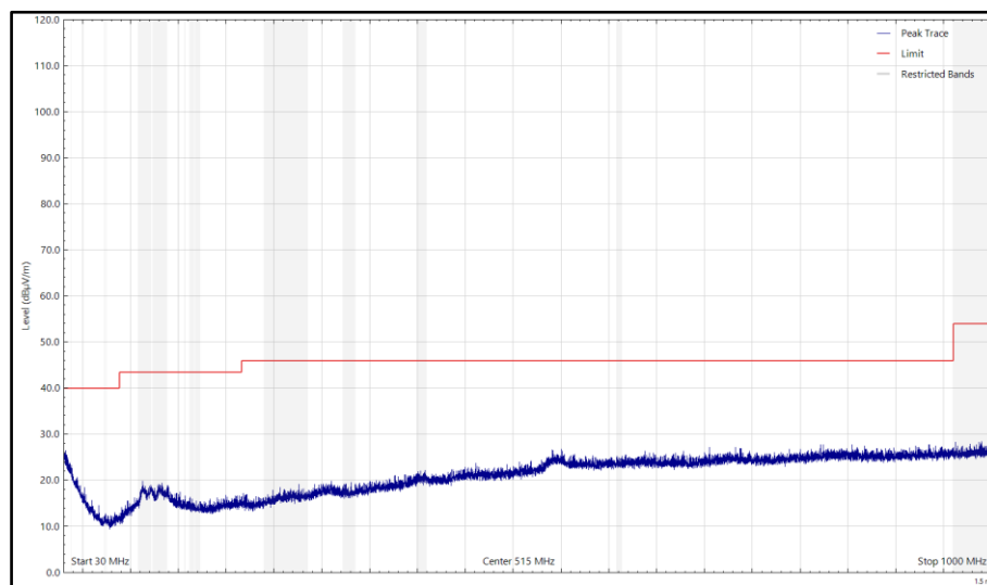
Figure 62- Bottom_2402 MHz, LE500k - 30 MHz to 1 GHz, Horizontal (Peak) Z- Orientation
