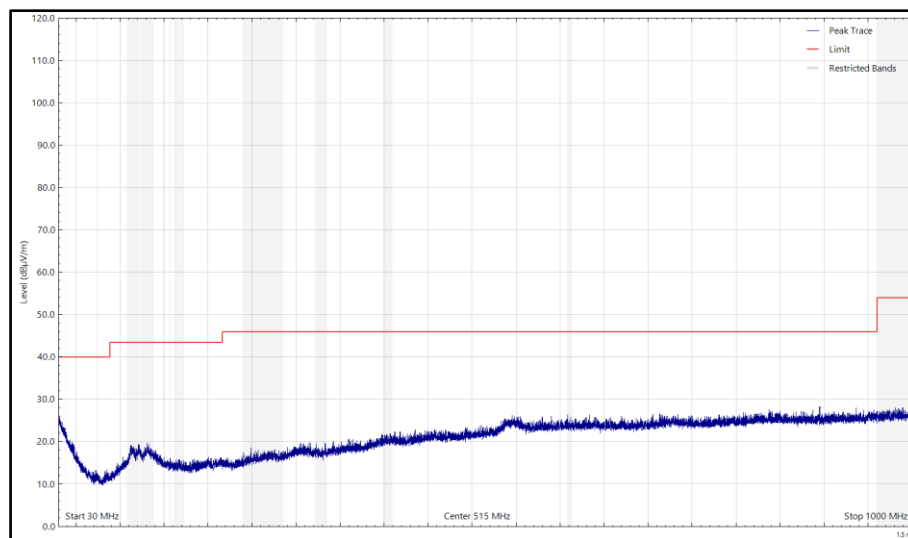
Figure 66- Mid_2440 MHz, LE500k - 30 MHz to 1 GHz, Horizontal (Peak) Z- Orientation
