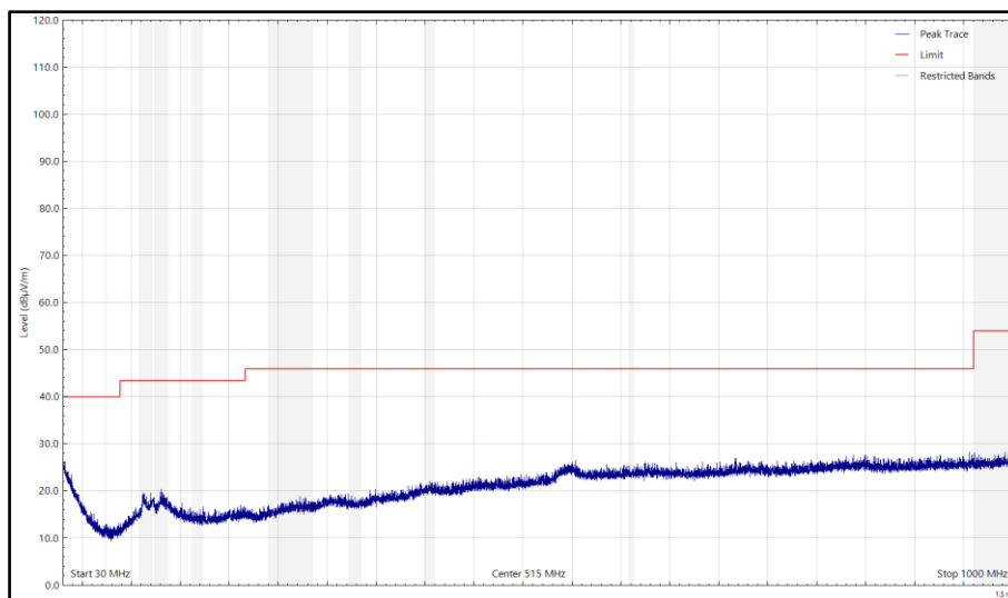
Figure 42- Mid_ 2440 MHz, LE500k - 30 MHz to 1 GHz, Horizontal (Peak) X-Orientation
