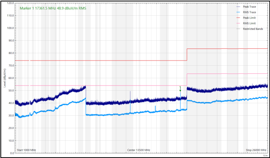
Figure 49 - Top_ 2480 MHz, LE500k - 1 GHz to 26 GHz, Vertical (Peak) X-Orientation
