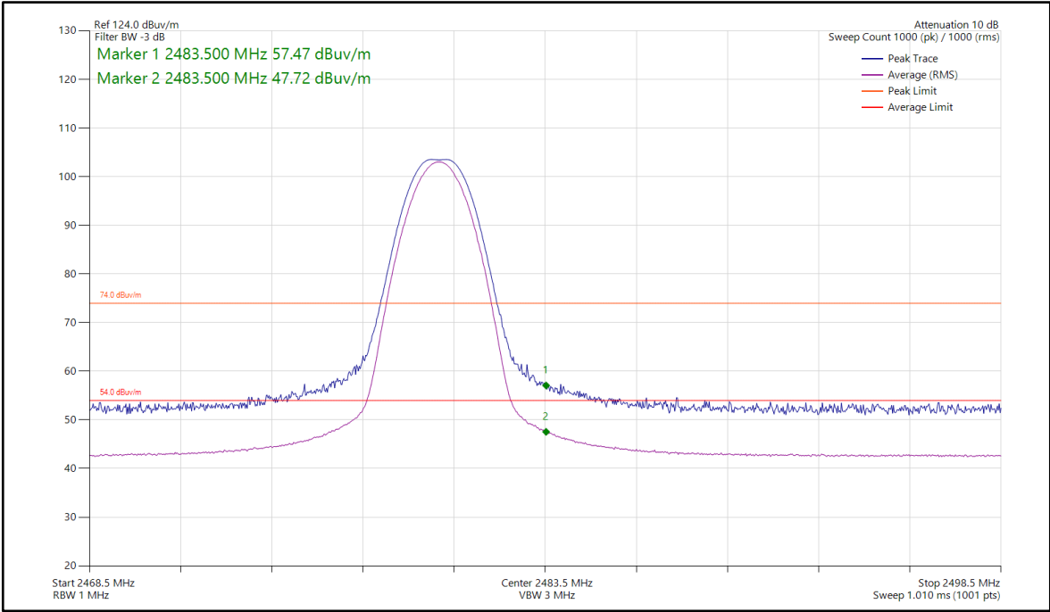
Figure 30 - TOP_BLE_1M_2480 MHz, Band Edge Frequency 2483.5 MHz
