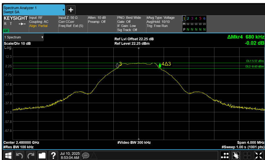
Figure 6 - 2480 MHz (CH39) 6 dB Bandwidth
