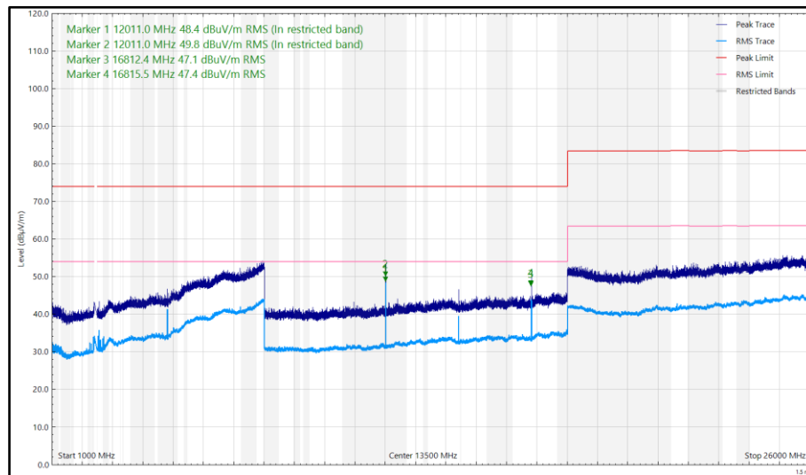
Figure 39- Bottom_ LE500k - 2402 MHz, 1 GHz to 26 GHz, Horizontal (Peak) X- Orientation
