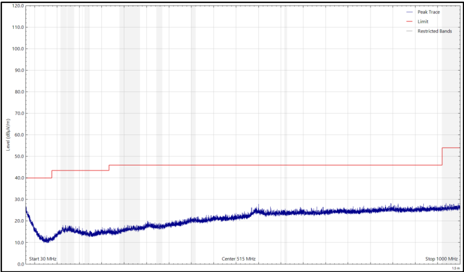
Figure 56- Mid_ 2402 MHz, LE500k - 30 MHz to 1 GHz, Vertical (Peak) Y- Orientation
