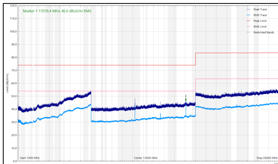
Figure 45- Mid_ 2440 MHz, LE500k - 1 GHz to 26 GHz, Vertical (Peak) X-Orientation
