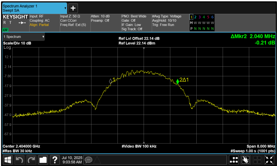
Figure 7 - 2404 MHz (CH37) 99% Bandwidth
