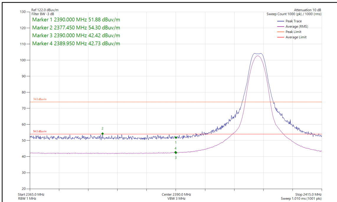
Figure 27 - BOT_BLE_2M_2404 MHz, Band Edge Frequency 2390 MHz
