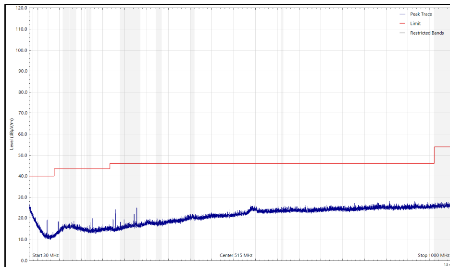
Figure 60- TOP_2480 MHz, LE500k - 30 MHz to 1 GHz, Vertical (Peak) Y-Orientation
