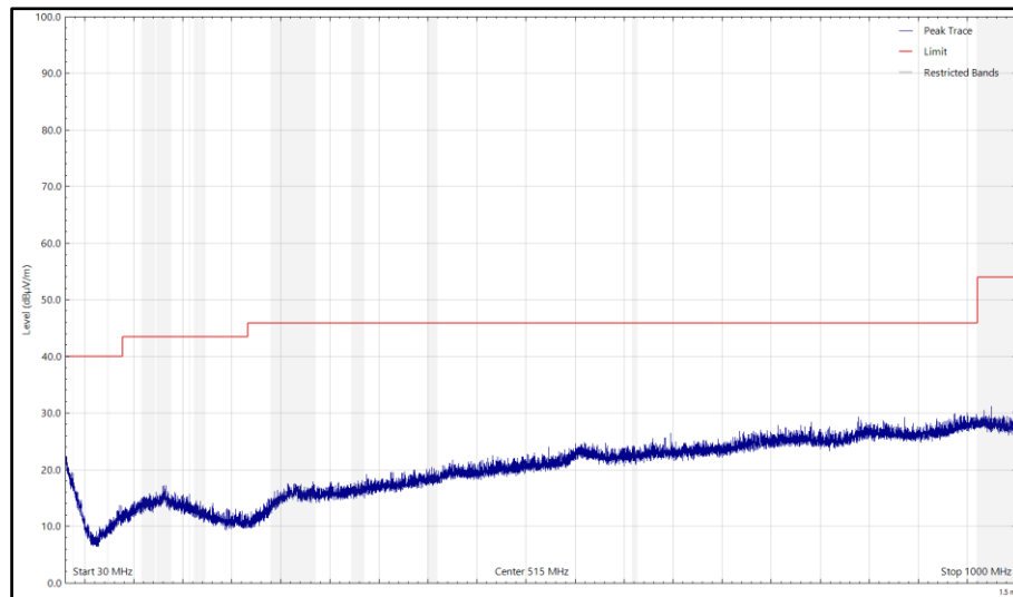
Figure 76 - Bottom _802.15.4_2405 MHz, 30 MHz to 1 GHz, Vertical (Peak) Z- Orientation
