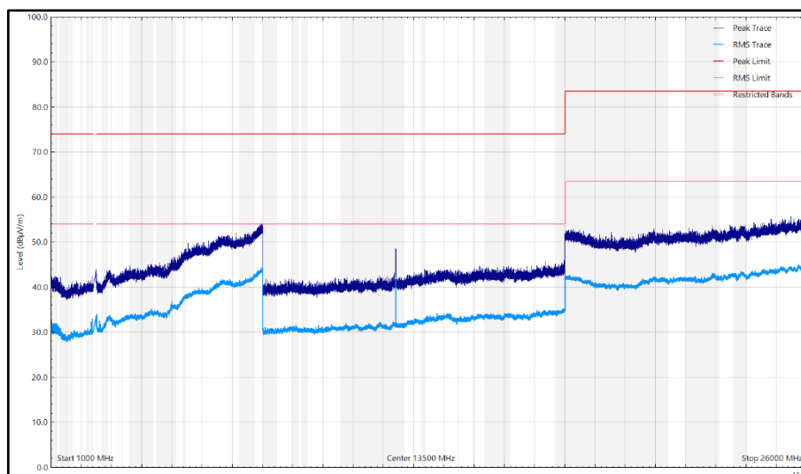
Figure 73 - Top _802.15.4_2480 MHz, 1 GHz to 26 GHz, Vertical (Peak) Y- Orientation
