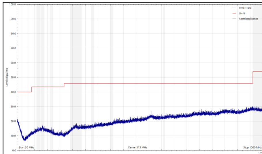
Figure 80 - Middle _802.15.4_2485 MHz, 30 MHz to 1 GHz, Vertical (Peak) Z- Orientation
