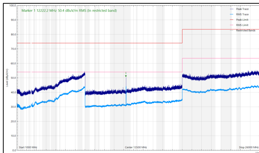
Figure 79 - Middle_802.15.4_2445 MHz, 1 GHz to 26 GHz, Horizontal (Peak) Z- Orientation
