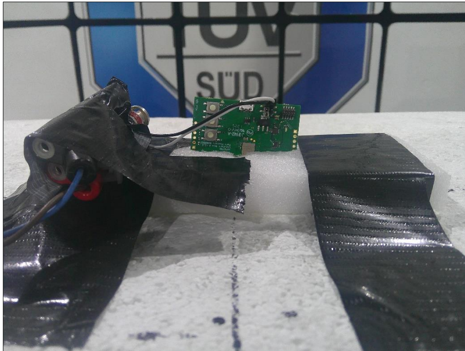
Figure 96 - Test Setup - Y - Orientation
