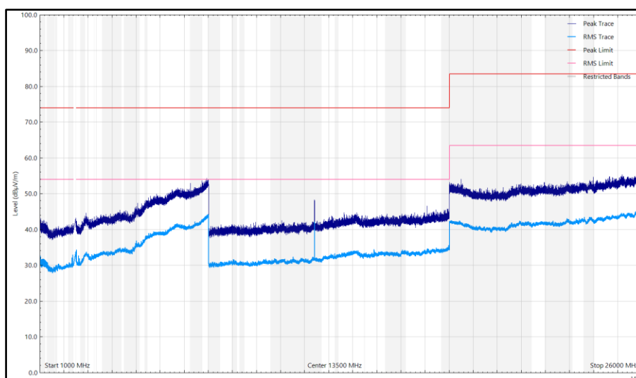
Figure 83 - Top_802.15.4_2480 MHz, 1 GHz to 26 GHz, Horizontal (Peak) Z- Orientation
