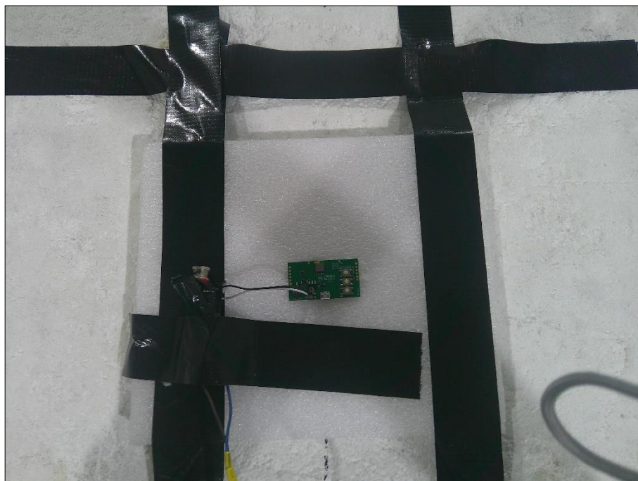
Figure 95 - Test Setup - X - Orientation
