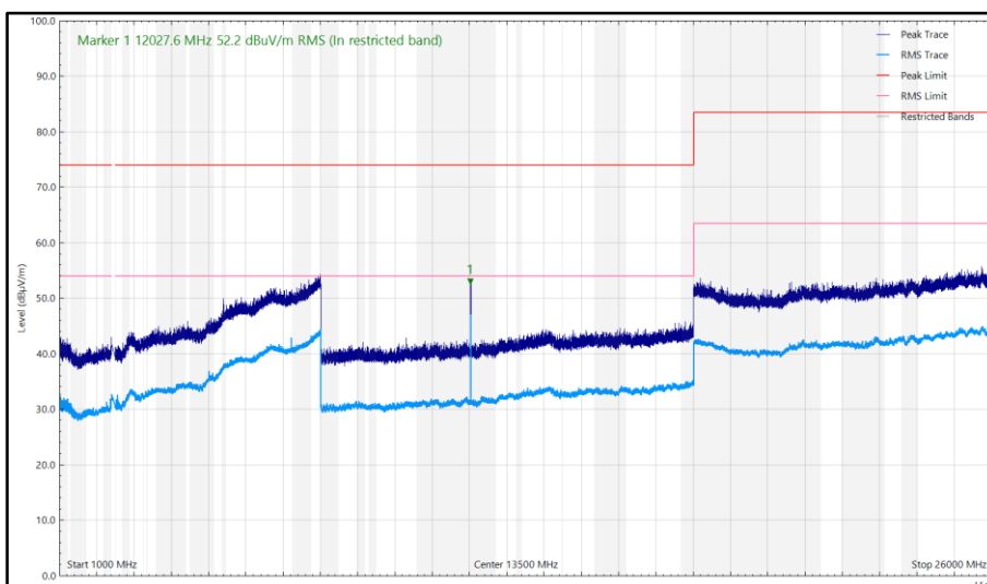
Figure 75 - Bottom_802.15.4_2405 MHz, 1 GHz to 26 GHz, Horizontal (Peak) Z- Orientation
