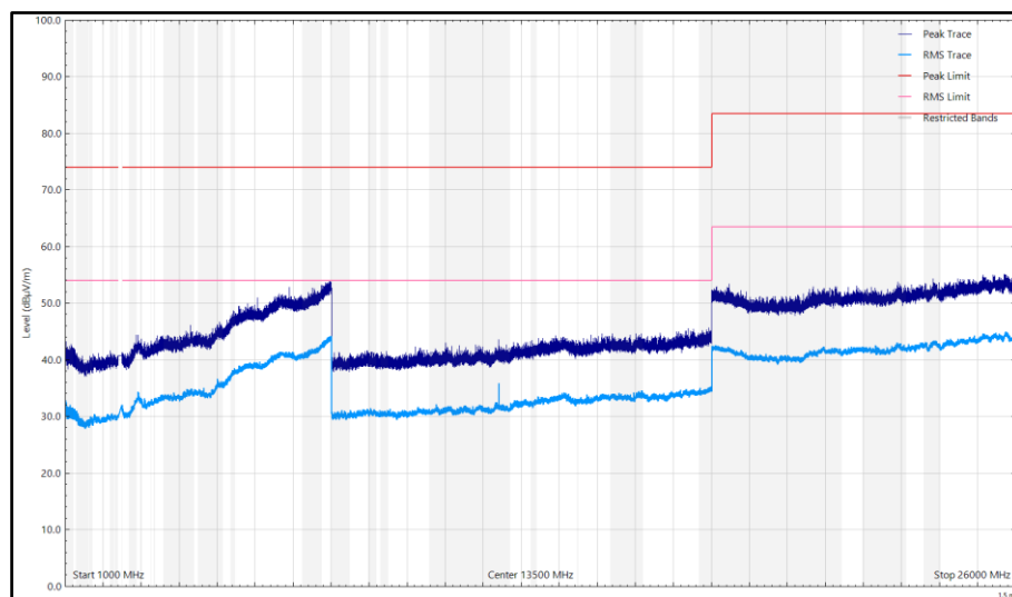
Figure 85 - Top _802.15.4_2480 MHz, 1 GHz to 26 GHz, Vertical (Peak) Z- Orientation
