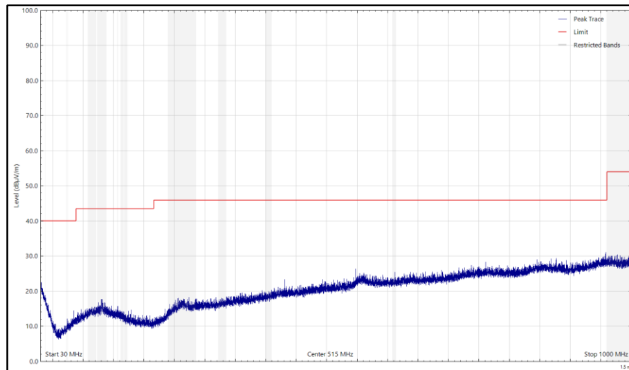
Figure 72 - Top _802.15.4_2480 MHz, 30 MHz to 1 GHz, Vertical (Peak) Y- Orientation
