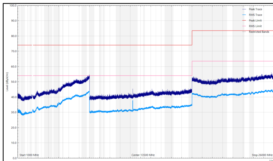
Figure 81 - Middle _802.15.4_2445 MHz, 1 GHz to 26 GHz, Vertical (Peak) Z- Orientation
