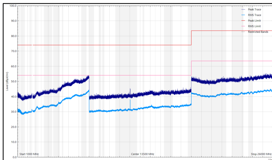
Figure 77 - Bottom _802.15.4_2405 MHz, 1 GHz to 26 GHz, Vertical (Peak) Z- Orientation
