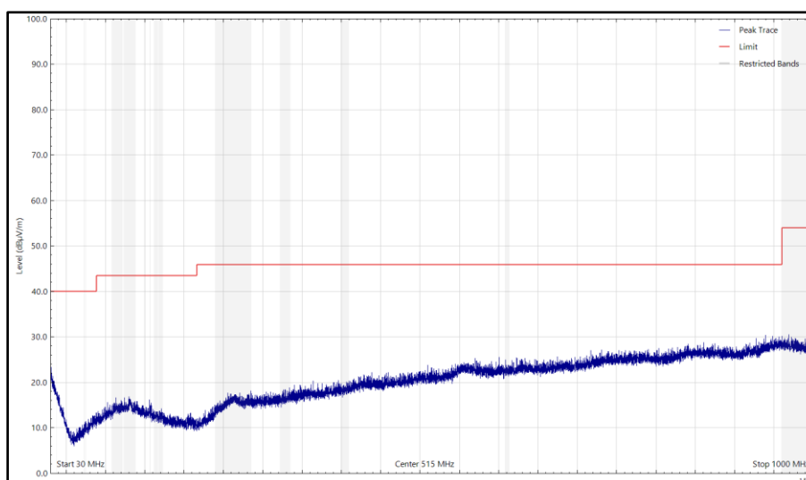
Figure 82 - Top_802.15.4_2480 MHz, 30 MHz to 1 GHz, Horizontal (Peak) Z- Orientation
