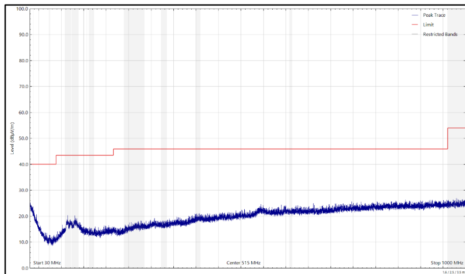
Figure 78 - Middle_802.15.4_2445 MHz, 30 MHz to 1 GHz, Horizontal (Peak) Z- Orientation
