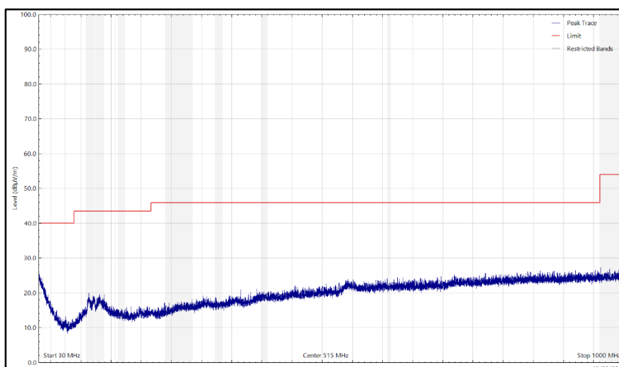
Figure 74 - Bottom_802.15.4_2405 MHz, 30 MHz to 1 GHz, Horizontal (Peak) Z- Orientation
