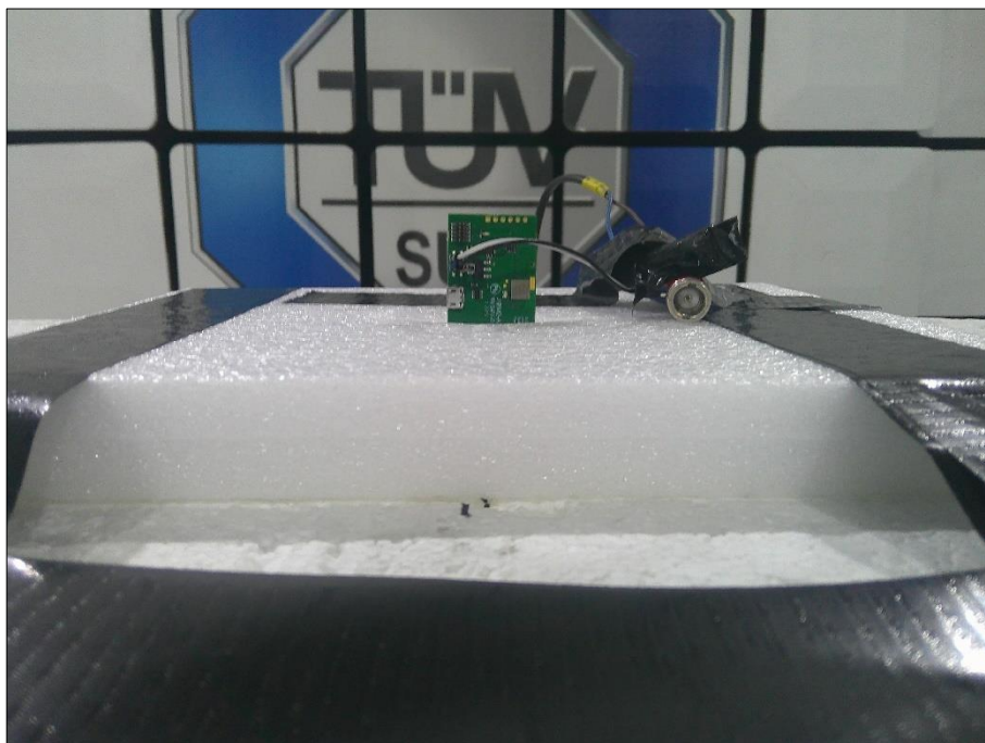
Figure 97 - Test Setup - Z - Orientation
