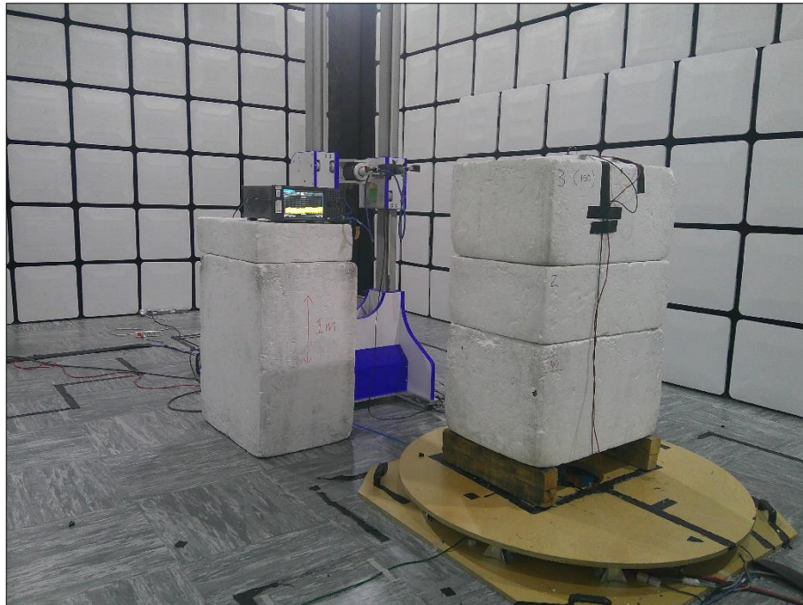
Figure 94 - Test Setup - 18 GHz to 26 GHz
