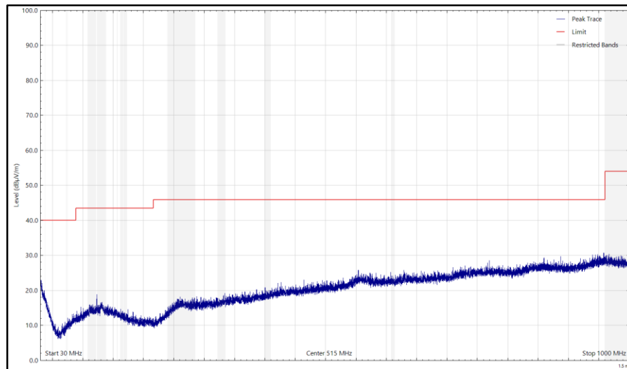
Figure 84 - Top _802.15.4_2480 MHz, 30 MHz to 1 GHz, Vertical (Peak) Z- Orientation
