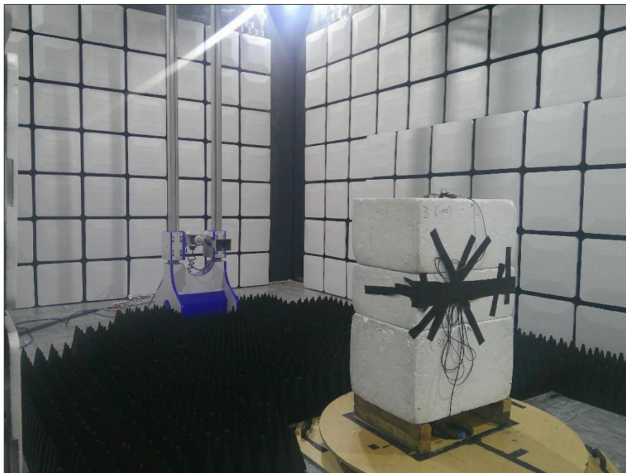
Figure 93 - Test Setup - 1 GHz to 18 GHz
