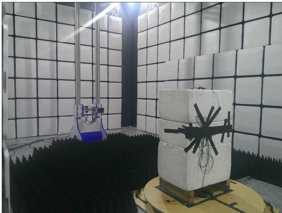
Figure 8 - Test Setup - 1 GHz to 18 GHz
