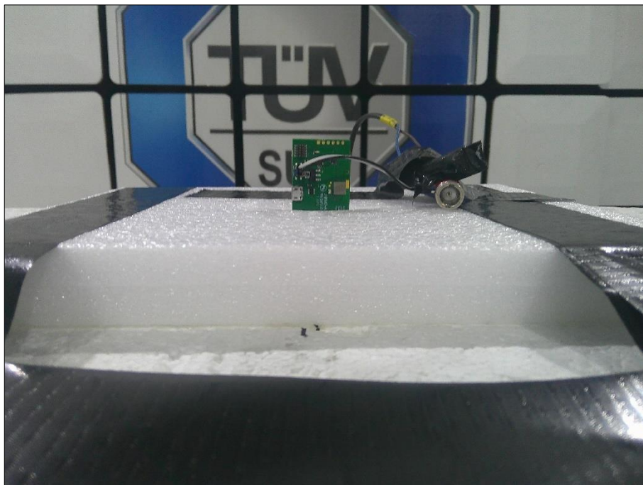
Figure 12 - Test Setup - Z- Orientation
