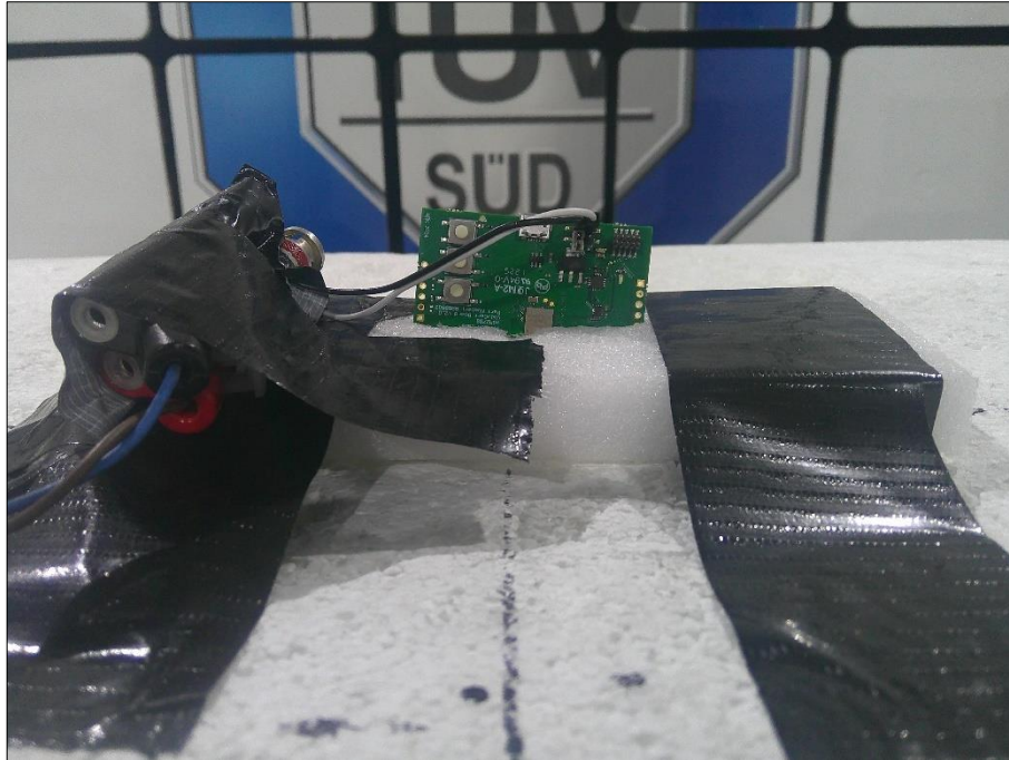
Figure 11 - Test Setup - Y- Orientation
