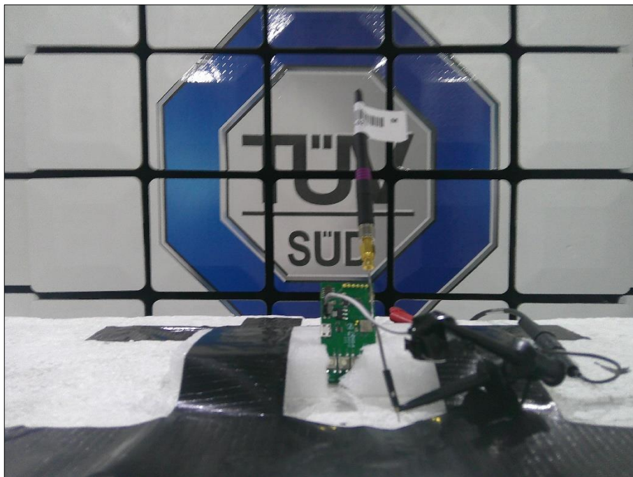
Figure 6 - Test Setup - Z - Orientation
