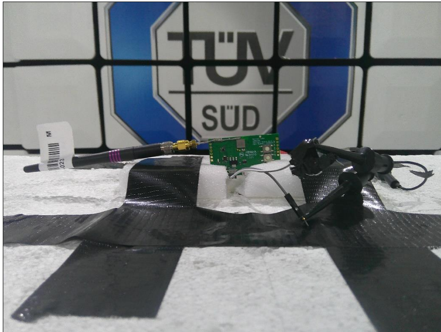
Figure 5 - Test Setup - Y- Orientation
