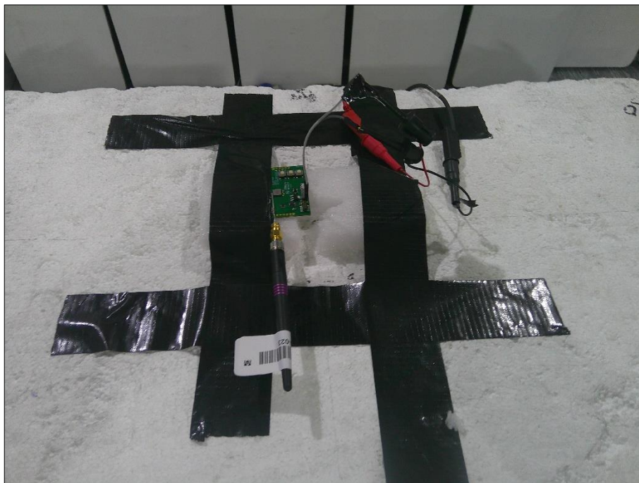
Figure 4 - Test Setup - X - Orientation
