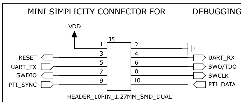
Figure 5.1. MGM240L Application Schematic
