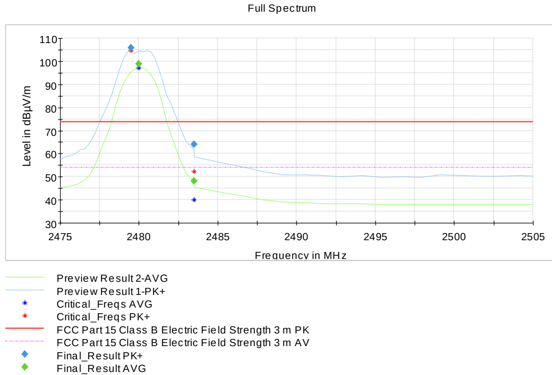
Figure 15: Radiated Band Edge measurement graph, Channel 26 high
