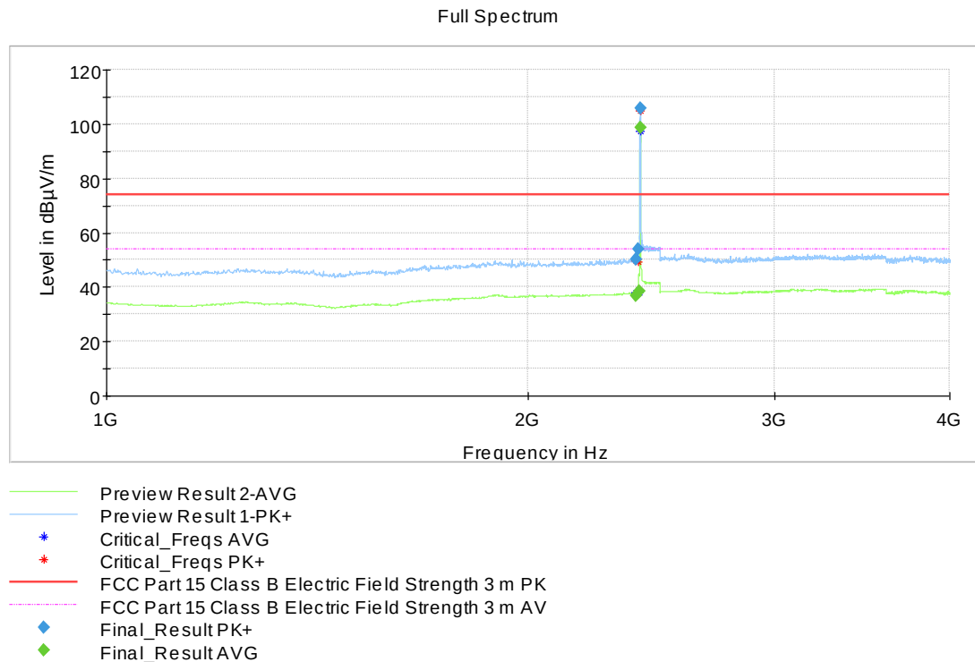
Figure 2: Channel 11 low 1 GHz – 4 GHz
