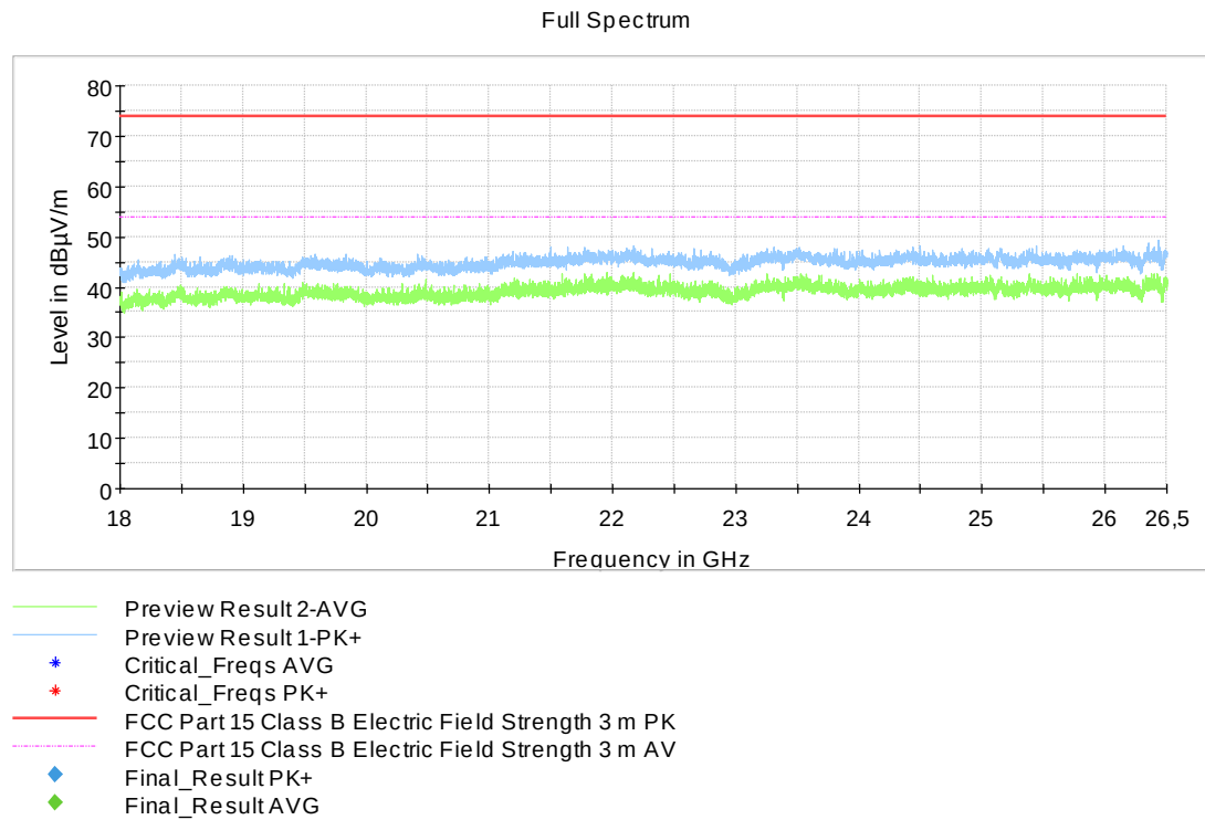
Figure 9: Channel 19 mid 18 GHz – 26.5 GHz
