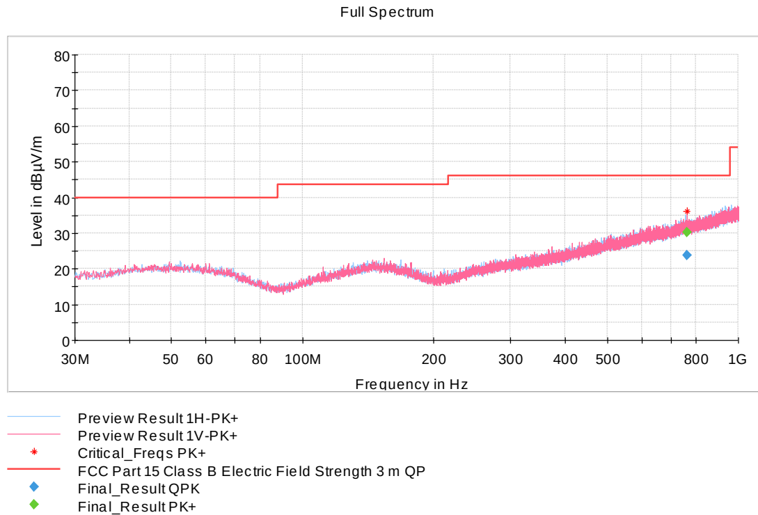
Figure 1: Channel 11 low 30 MHz – 1000 MHz
