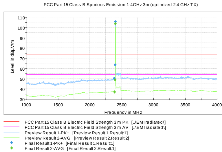
Figure 6: Low channel 1 GHz – 4 GHz (A)
