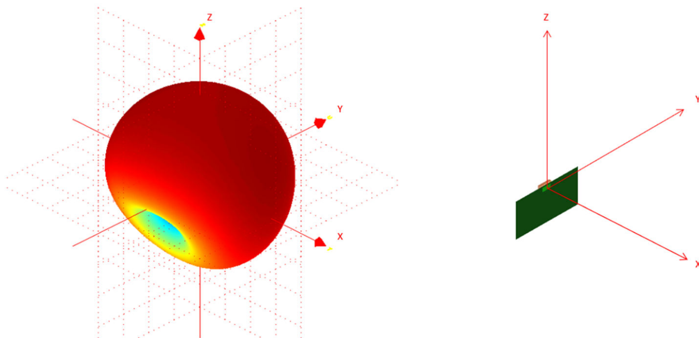
Figure 3.11. 3D Radiation Pattern of the Build-In Antenna
