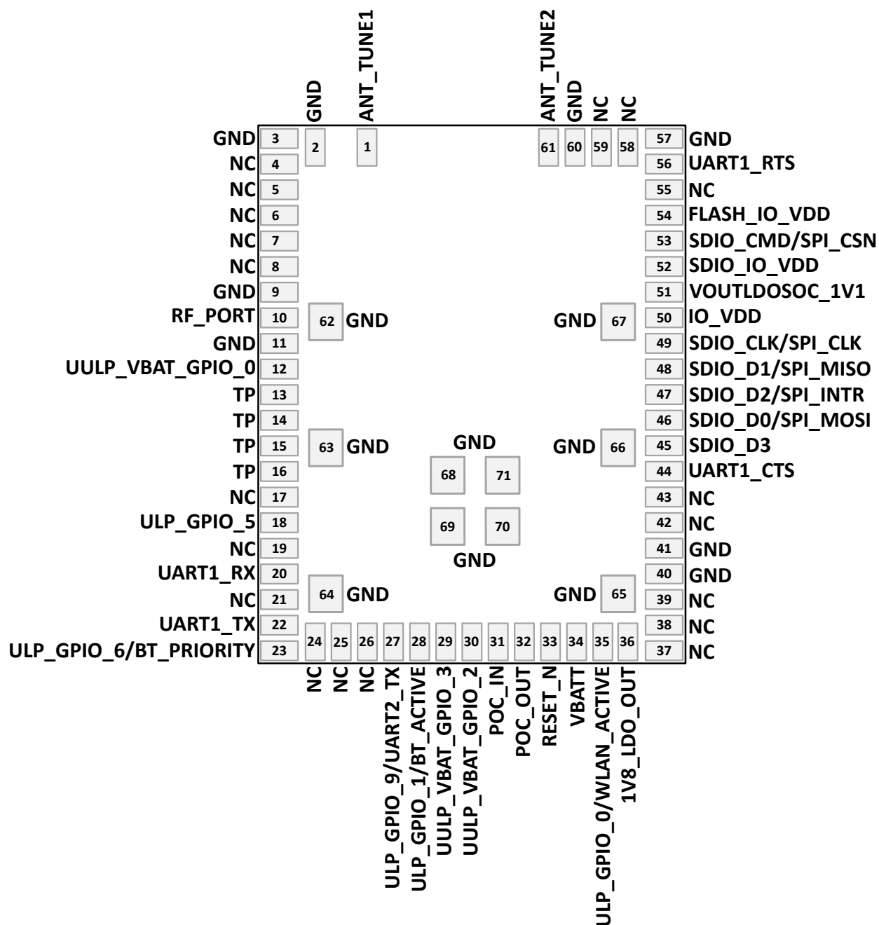
Figure 1.1. RS916AC0 and RS916AC1 Pin Diagram
