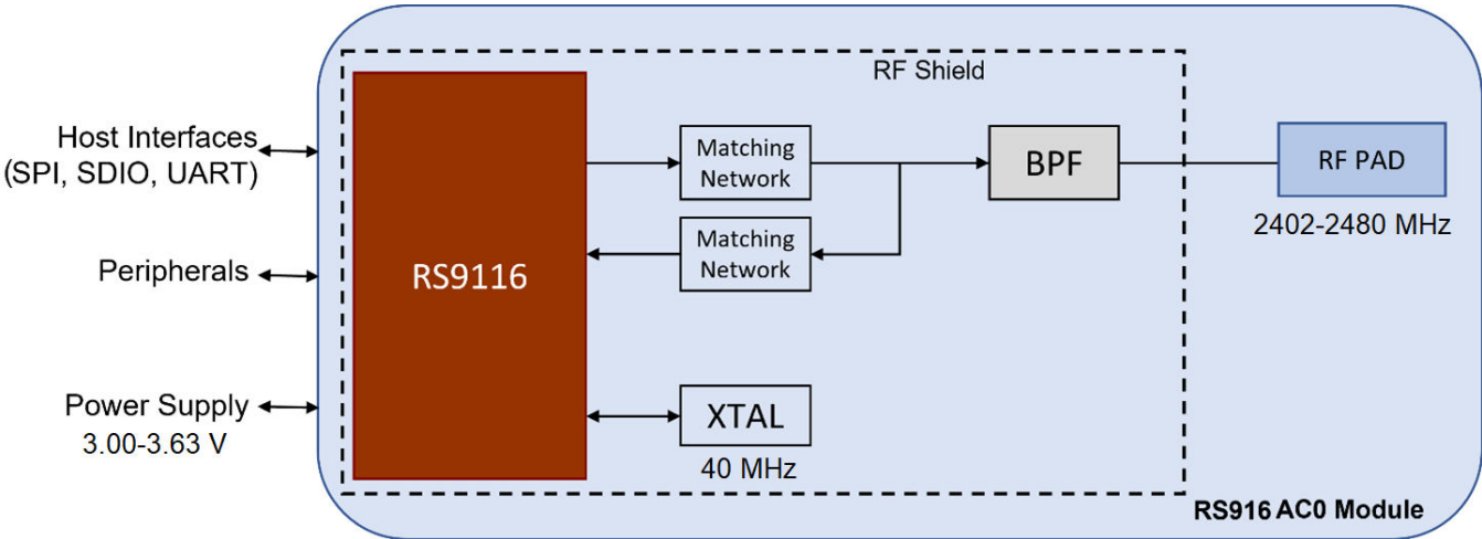
RS916AC0 Module Block Diagram
