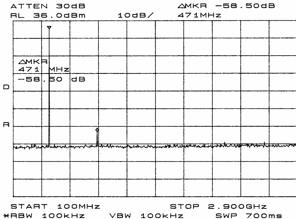
Figure 11: Emissions at Antenna Terminal (4W)
