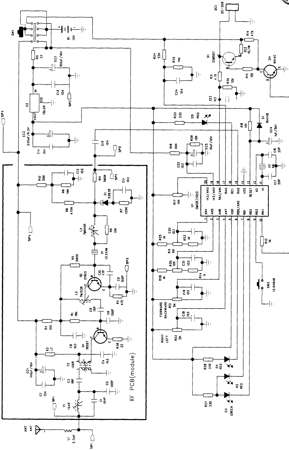
CPU PCB
