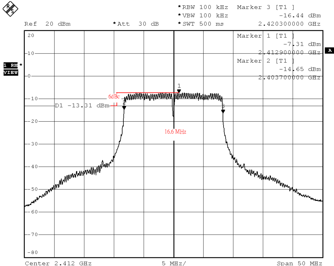
Figure Channel 1:
