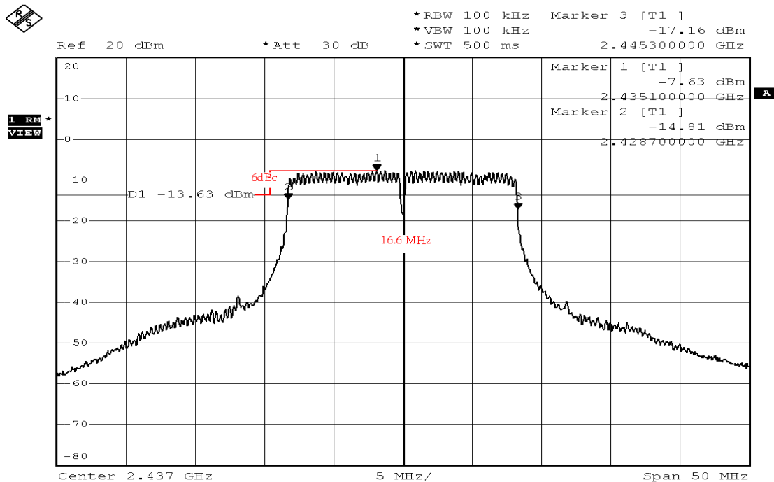
Figure Channel 6:
