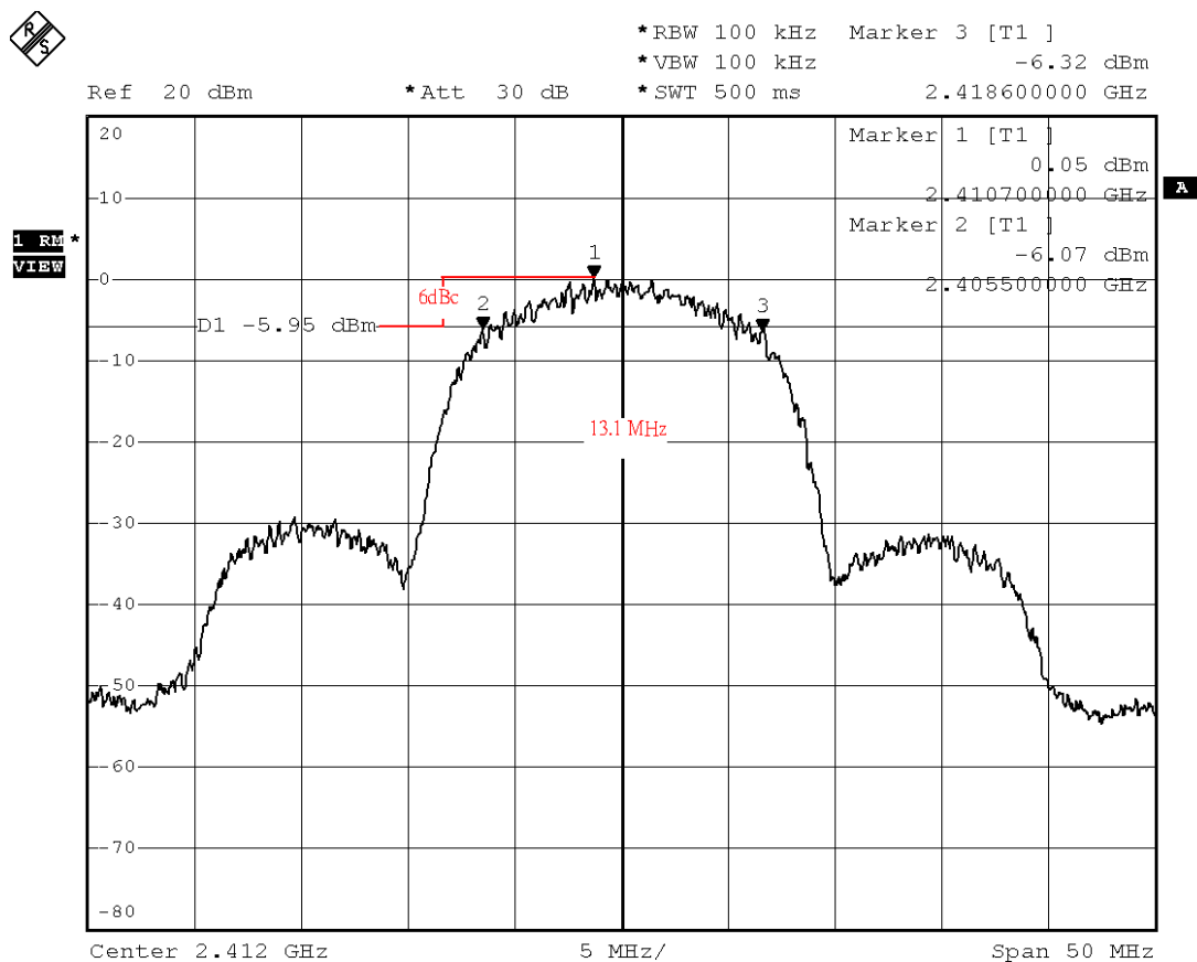
Figure Channel 1:
