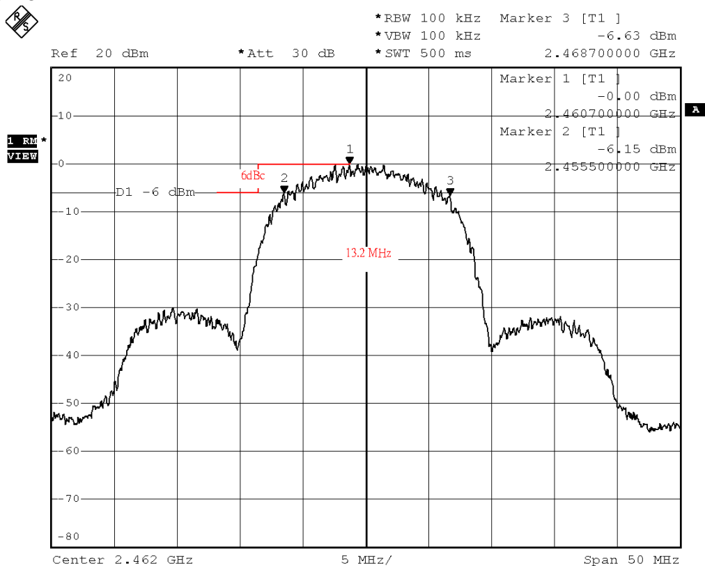
Figure Channel 11:
