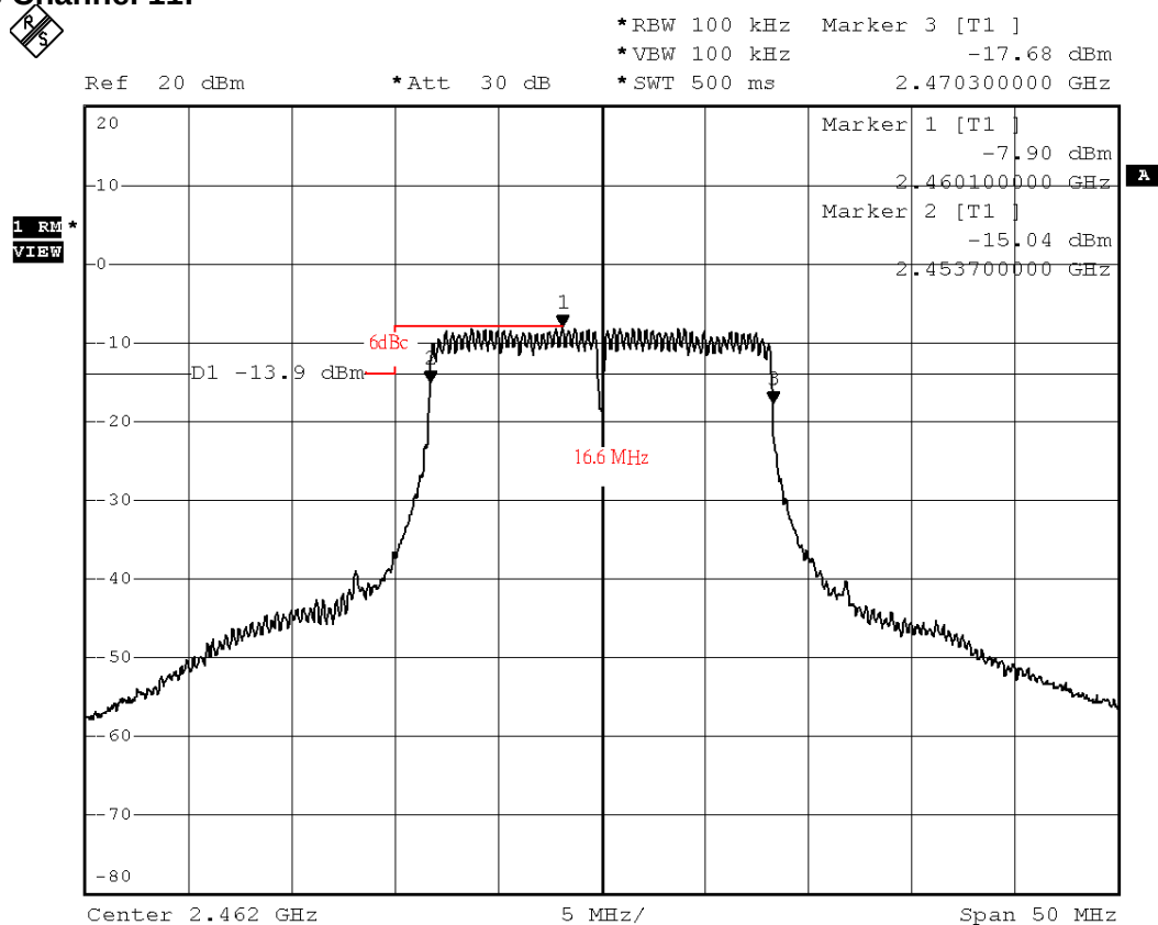
Figure Channel 11:
