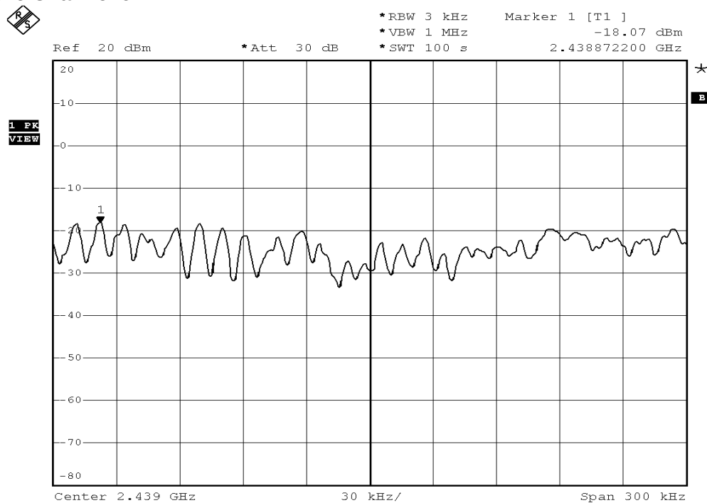
Figure Channel 6:
