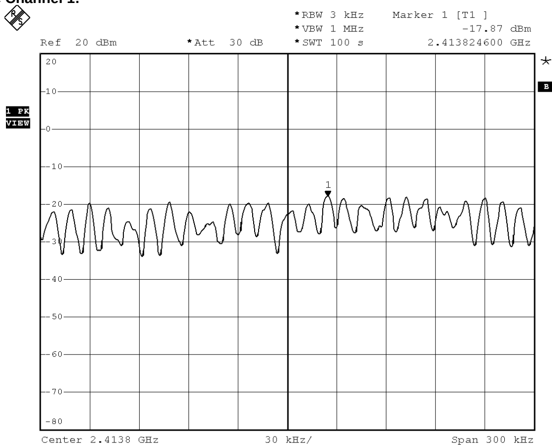
Figure Channel 1:
