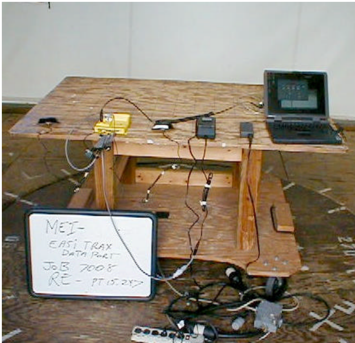
Radiated Emissions Test Configuration – Rear View
