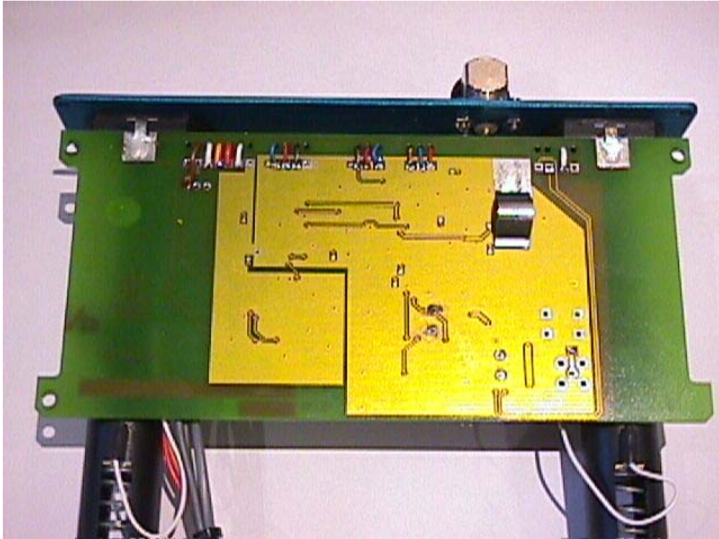
AQUA FM TX PRO – PCB back side internal view and rear panel
