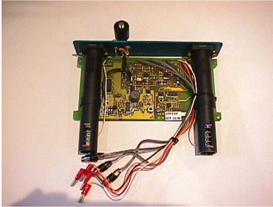
AQUA FM TX PRO –Internal view with PCB and rear panel
