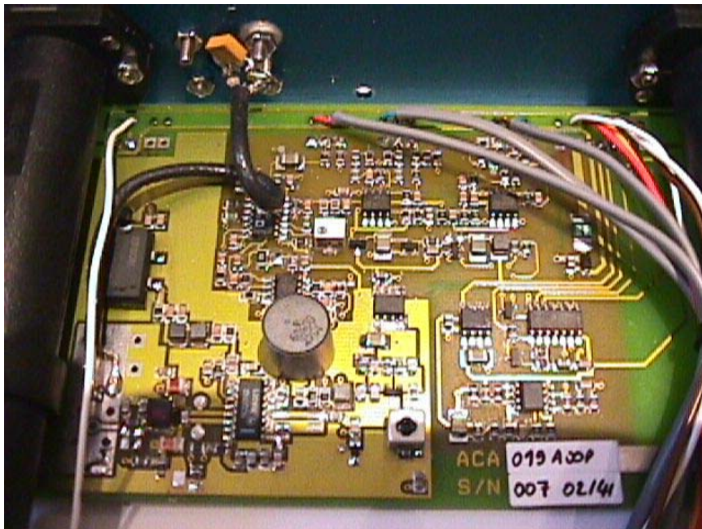
AQUA FM TX PRO – PCB components side internal detail view
