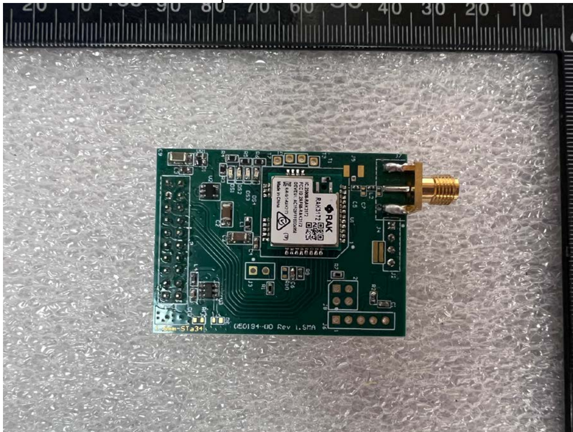
EUT/ Wireless Module PCB Component Side
