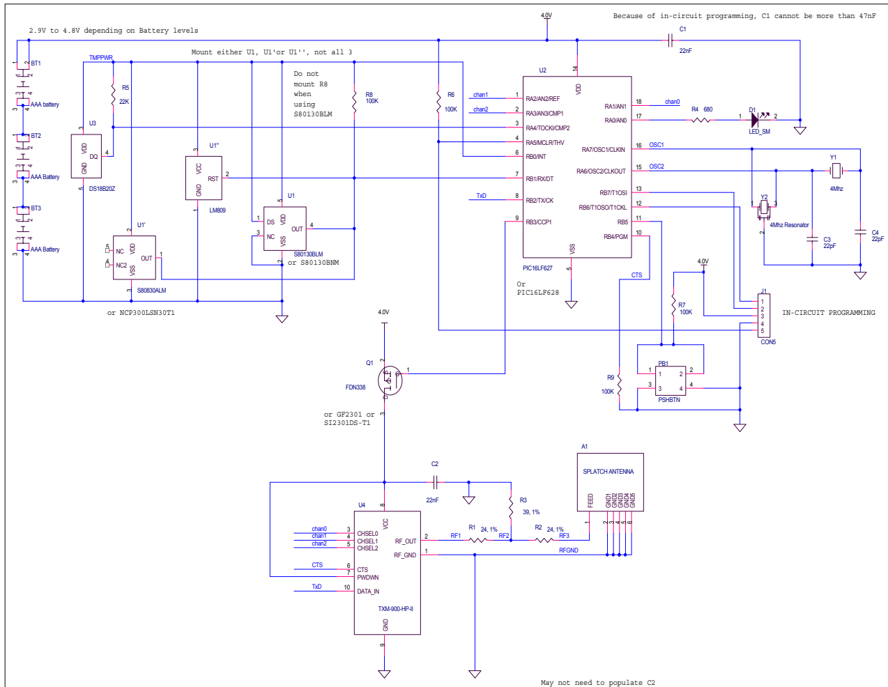
Sensor Link Room Temperature Transmitter Schematic Diagram
