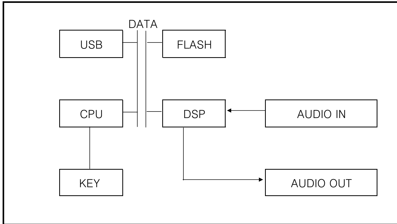
DVR+MP3 BLOCK DIAGRAM
