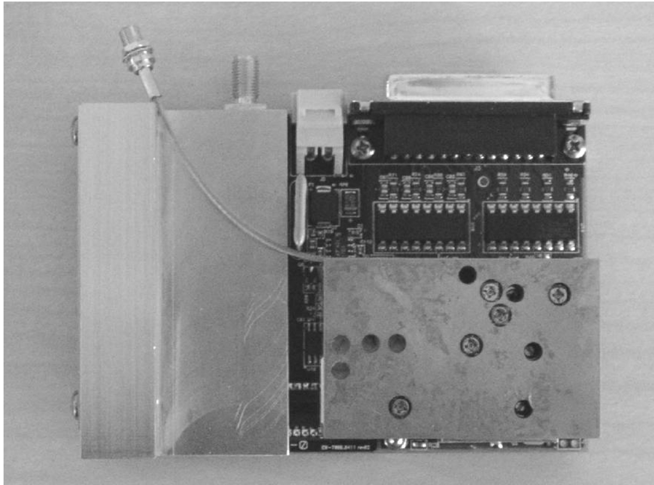
EVERYDAY WIRELESS TX-3 – INTERNAL TOP VIEW
