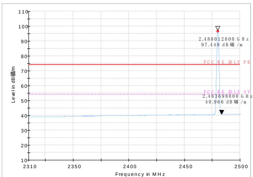
Fig.25 Bandedge: Ch39
