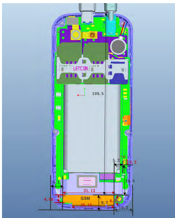
Fig.13 Antenna position of EUT
