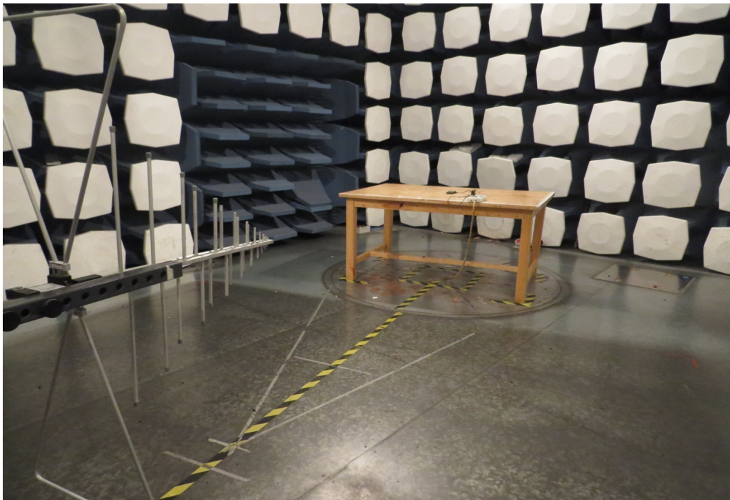
Below 1GHz
