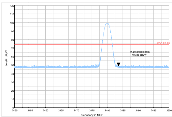
DH5-Channel 78: Peak
