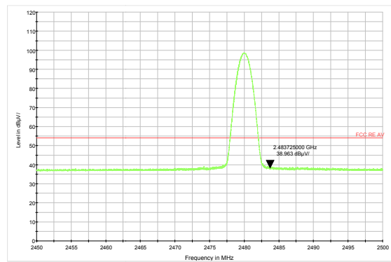
DH5-Channel 78: Average
