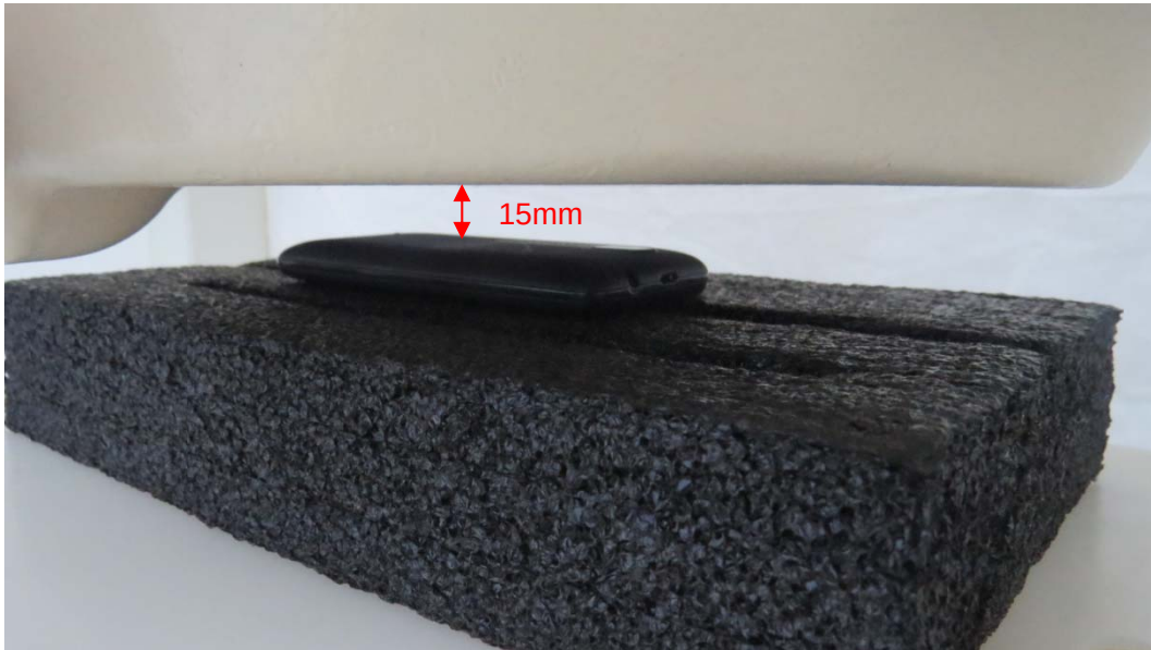
Picture 7: Back Side, the distance from handset to the bottom of the Phantom is 15mm
