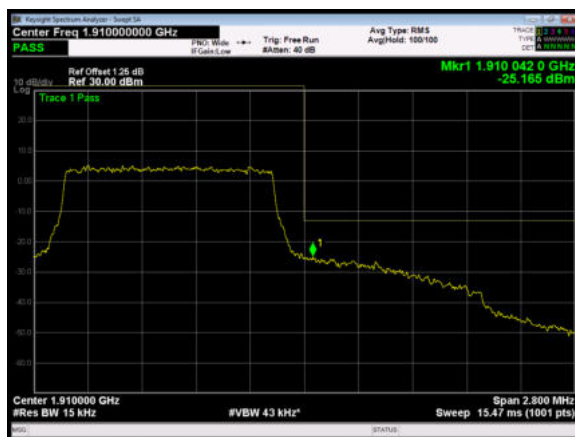
LTE Band 2 1.4MHz QPSK 100%RB CH-High
