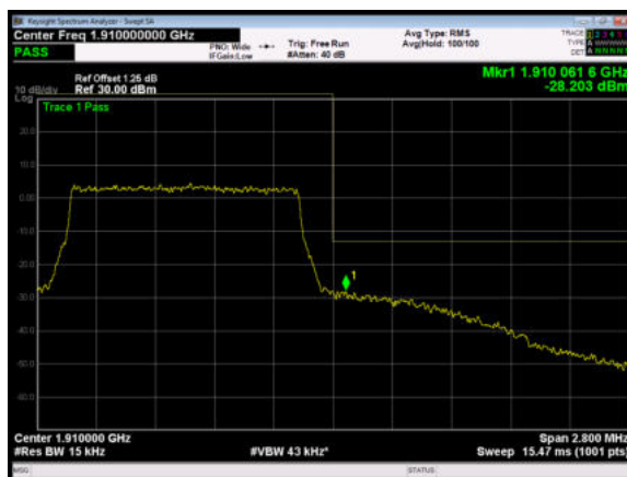
LTE Band 2 3MHz 16QAM 1RB CH-High
