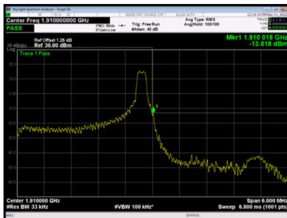
LTE Band 2 3MHz 16QAM 100%RB CH-High
