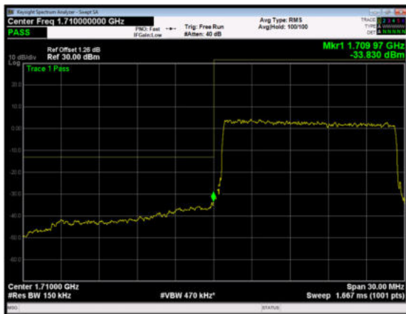
LTE Band 4 QPSK 20MHz CH-Low, 1 RB
