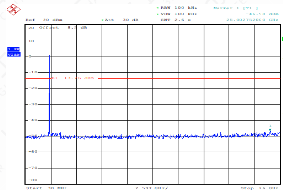
(802.11g, Ch11, 30MHz~26GHz)
