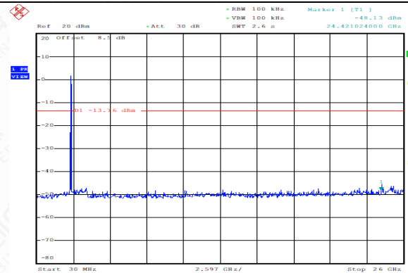
Conducted Spurious Emission (802.11n-20MHz, Ch6, 30MHz~26GHz)
