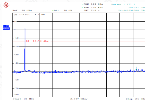
(802.11g, Ch6, 30MHz~26GHz)
