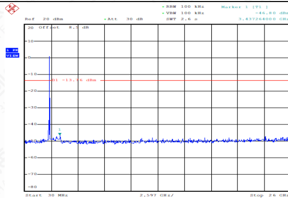
Conducted Spurious Emission (802.11n-20MHz, Ch1, 30MHz~26GHz)
