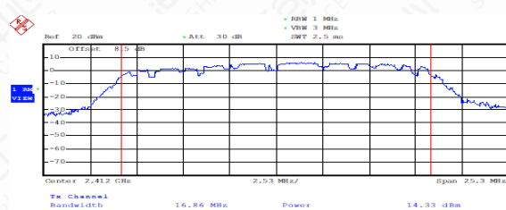
Output Power-Conducted (802.11g, Ch1)
