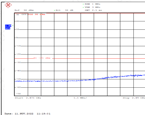
LowRange_FDD07_15MHz_2507.5_fullRB _Low_QPSK
