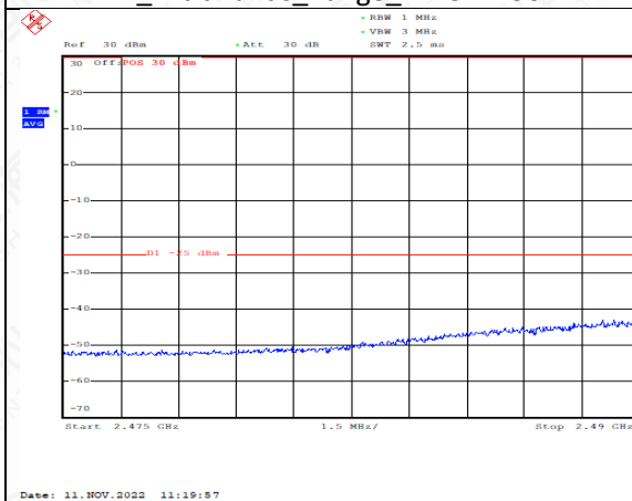
LowRange_FDD07_20MHz_2510_fullRB _Low_QPSK
