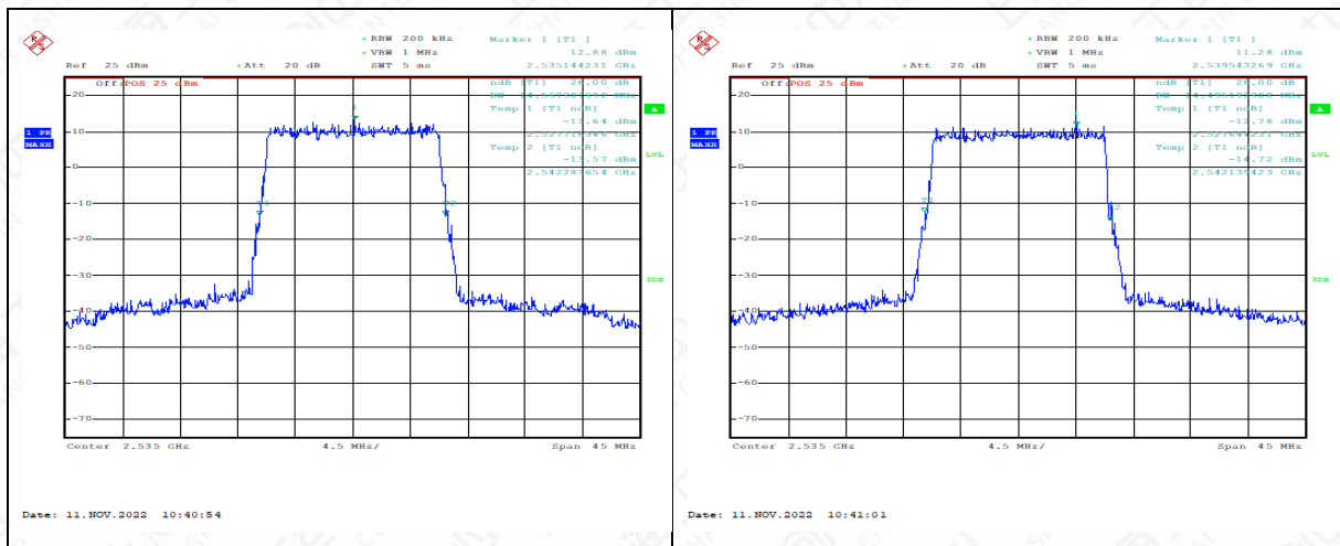
LTE band 7, 20MHz (-26dBc)mid
