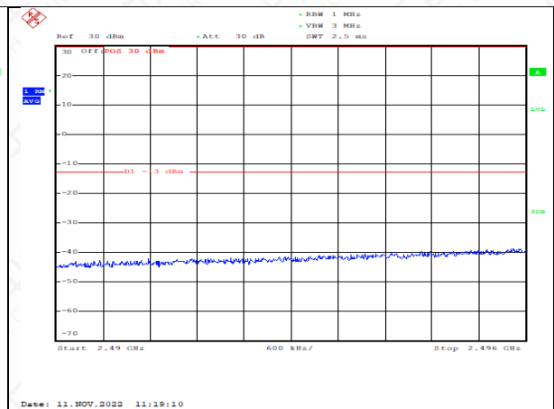
LowRange_FDD07_15MHz_2507.5_fullRB _Low_Q16
