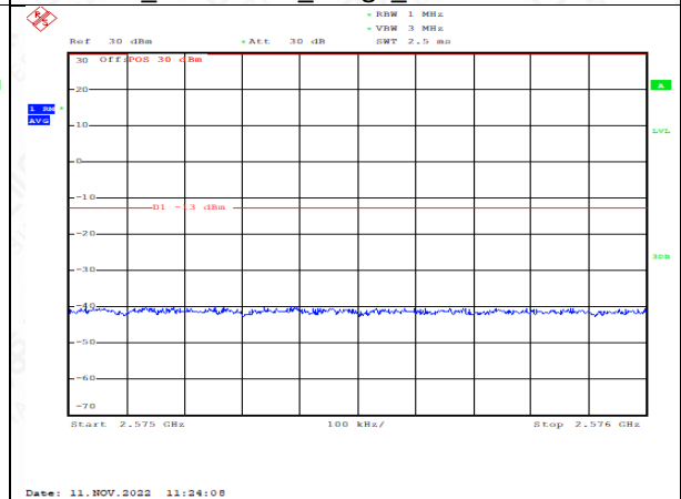
HighRange_FDD07_20MHz_2560_fullIRB _High_QPSK
