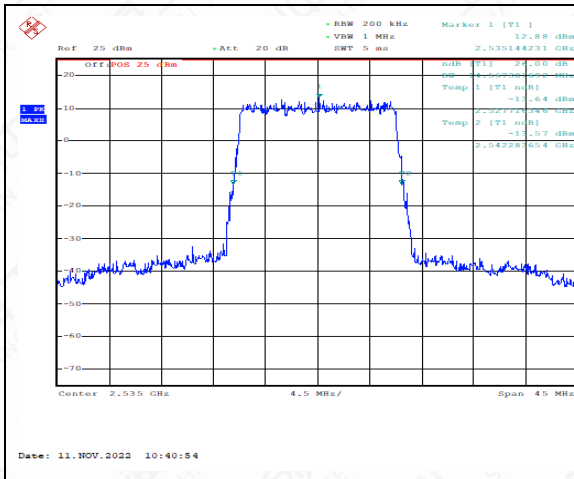
LTE band 7, 20MHz (99%)mid
