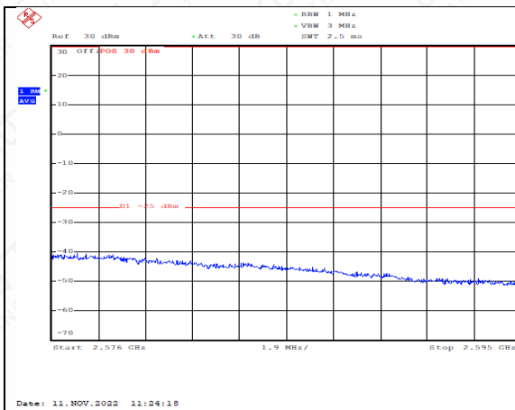
HighRange_FDD07_20MHz_2560_fullIRB_High_Q16
