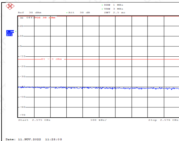
HighRange_FDD07_15MHz_2562.5_fullIRB _High_QPSK
