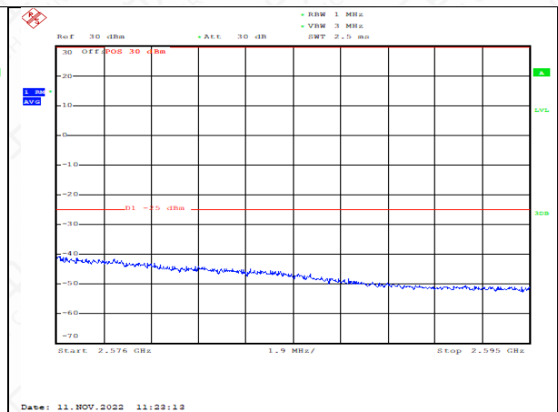
HighRange_FDD07_15MHz_2562.5_fullIRB _High_Q16
