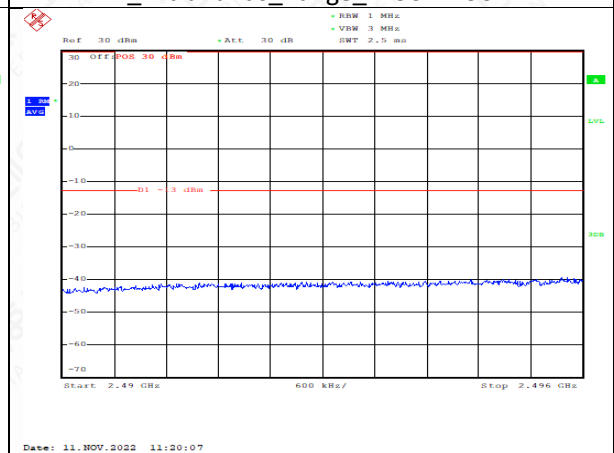
LowRange_FDD07_20MHz_2510_fullRB _Low_Q16
