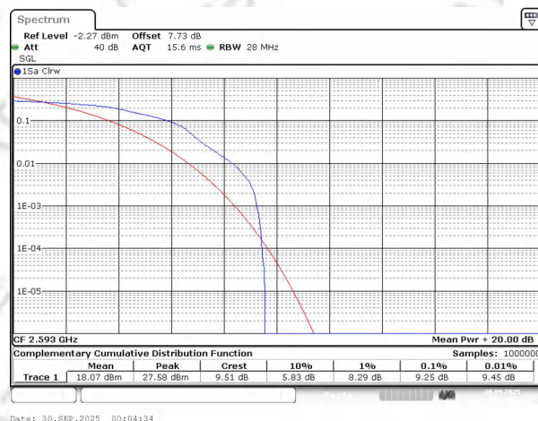
Band41 QAM16 BW=10MHz Channel=40620 RB Size=1 Position=#0 NVNT
