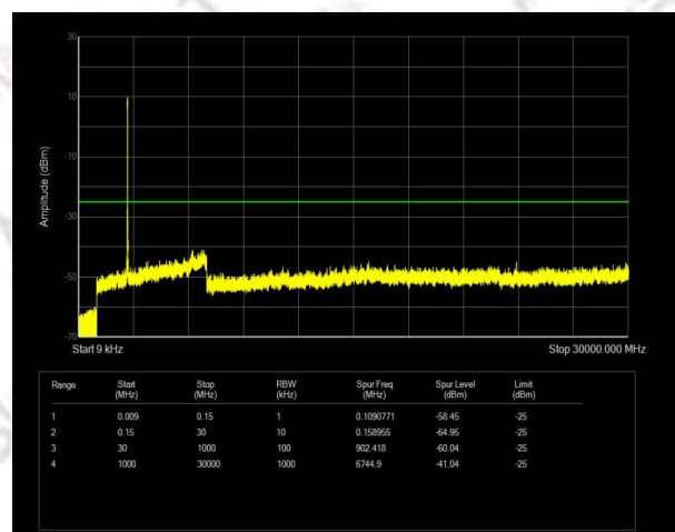
Band41 QAM16 BW=15MHz Channel=41515 RB Size=75 Position=#0 NVNT
