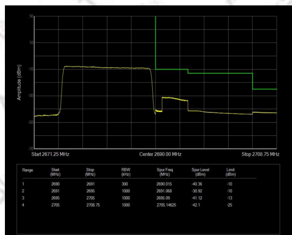
Band41 QAM16 BW=15MHz Channel=41515 RB Size=75 Position=#0 NVNT
