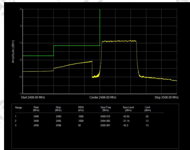
Band41 QAM16 BW=5MHz Channel=39675 RB Size=25 Position=#0 NVNT
