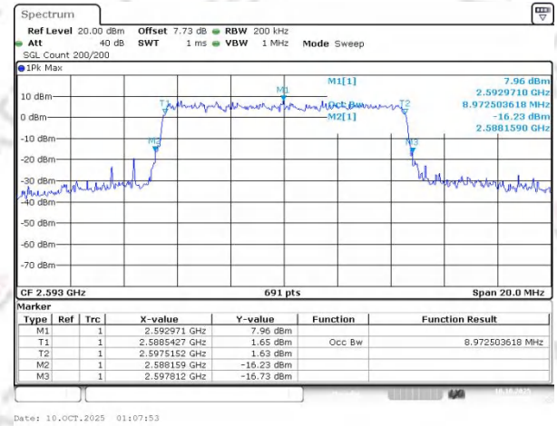
Band41 QAM16 BW=10MHz Channel=40620 RB Size=50 Position=#0
