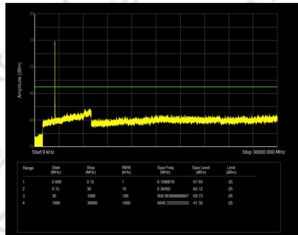
Band41 QAM16 BW=15MHz Channel=39725 RB Size=75 Position=#0 NVNT
