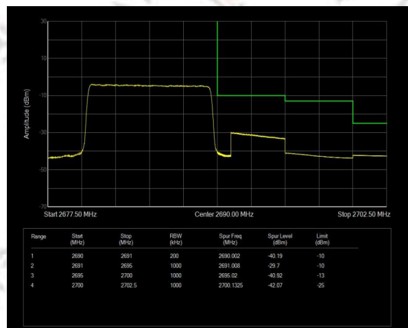
Band41 QAM16 BW=10MHz Channel=41540 RB Size=50 Position=#0 NVNT
