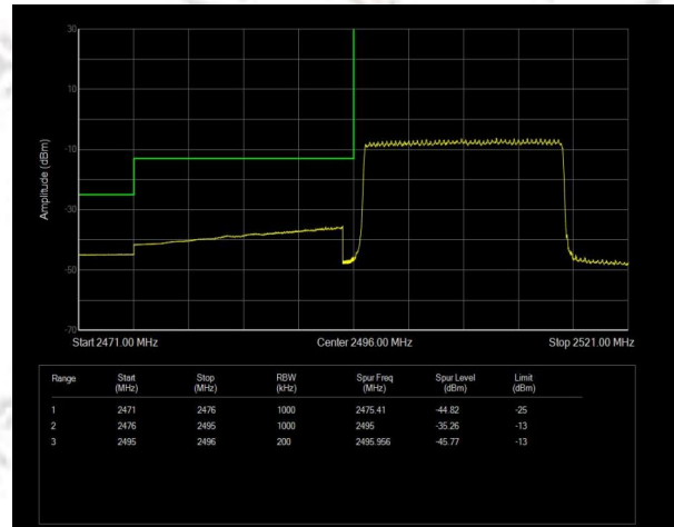
Band41 QAM16 BW=20MHz Channel=39750 RB Size=100 Position=#0 NVNT
