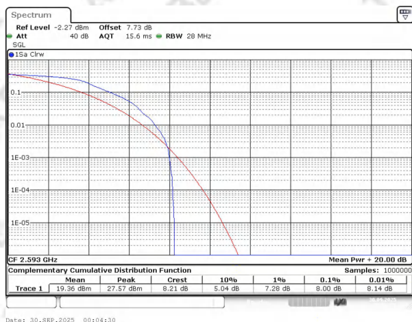
Band41 QPSK BW=10MHz Channel=40620 RB Size=1 Position=#0 NVNT
