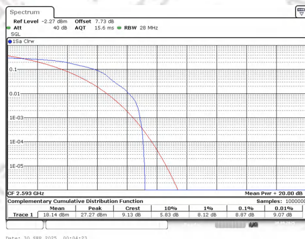
Band41 QAM16 BW=5MHz Channel=40620 RB Size=1 Position=#0 NVNT
