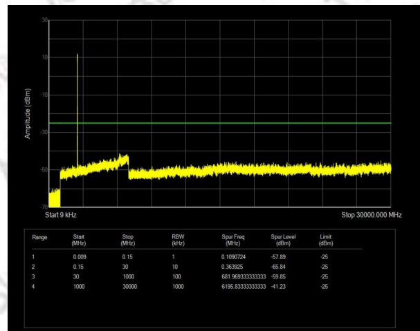
Band41 QAM16 BW=10MHz Channel=39700 RB Size=50 Position=#0 NVNT
