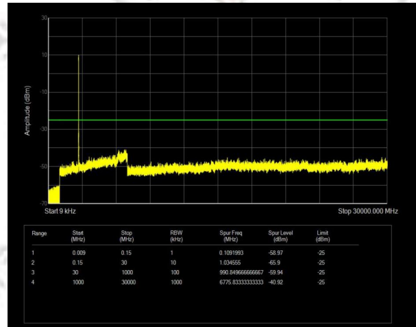
Band41 QAM16 BW=10MHz Channel=41540 RB Size=50 Position=#0 NVNT
