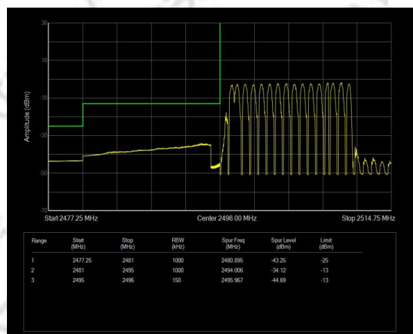
Band41 QAM16 BW=15MHz Channel=39725 RB Size=75 Position=#0 NVNT
