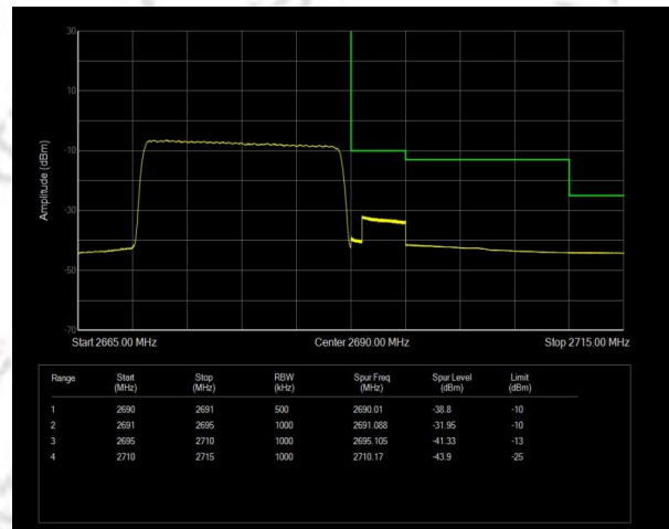
Band41 QAM16 BW=20MHz Channel=41490 RB Size=100 Position=#0 NVNT
