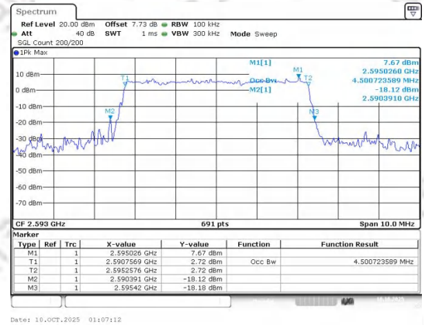
Band41 QAM16 BW=5MHz Channel=40620 RB Size=25 Position=#0 NVNT
