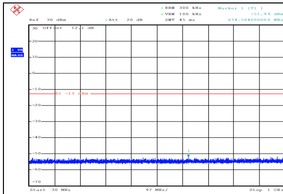
GSM1900_EDGE_661_30MHz-1000MHz _CSE
