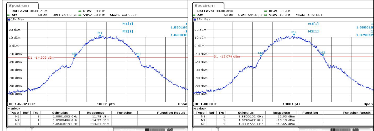
GSM1900,EDGE,5,1850.2MHz_OBW
