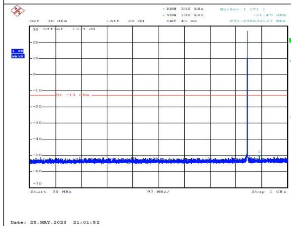
GSM850_EDGE_128_30MHz-1000MHz_CSE
