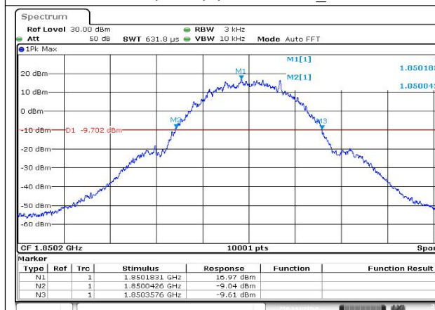
GSM1900,GSM,0,1850.2MHz_OBW
