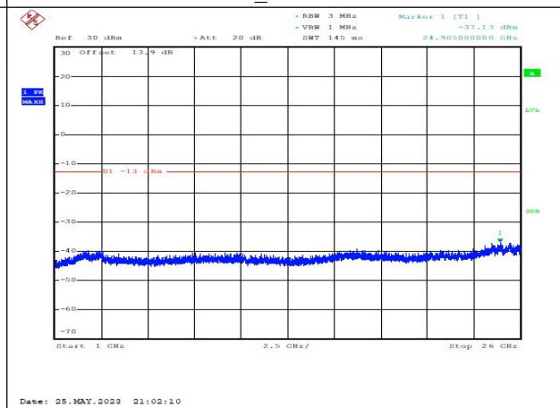
GSM850_EDGE_128_1000MHz-26000MHz_CSE
