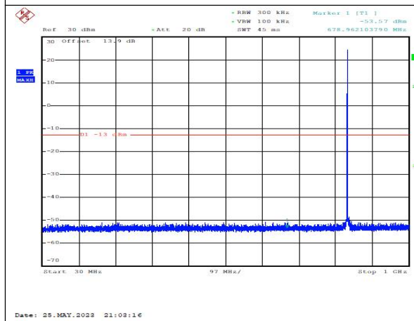
GSM850_EDGE_251_30MHz-1000MHz_CSE
