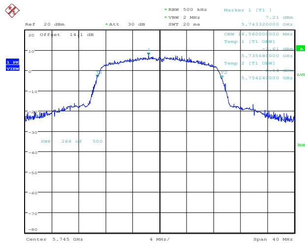
11N20SISO_Ant1_5745
