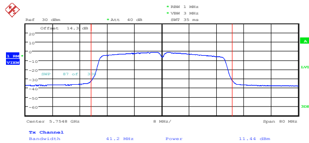
11AC40SISO_Ant1_5755
