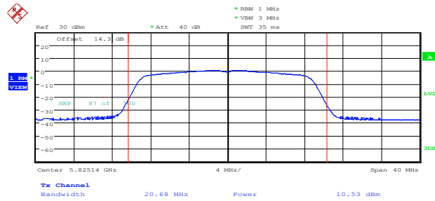
11N20SISO_Ant1_5825
