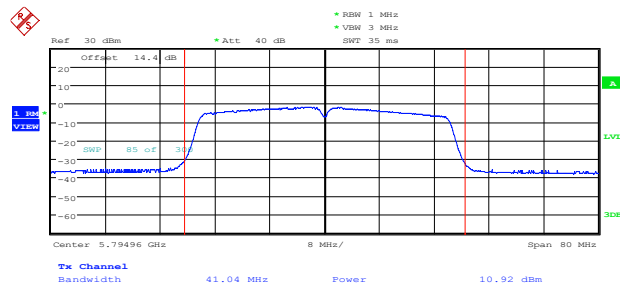
11N40SISO_Ant1_5795
