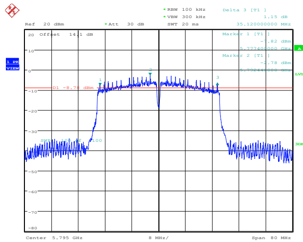
11N40SISO_Ant1_5795
