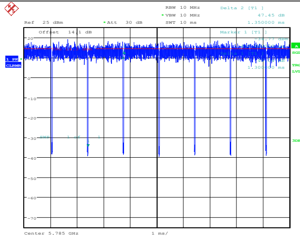
11N20SISO_Ant1_5785
