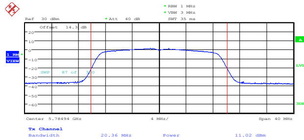
11AC20SISO_Ant1_5785
