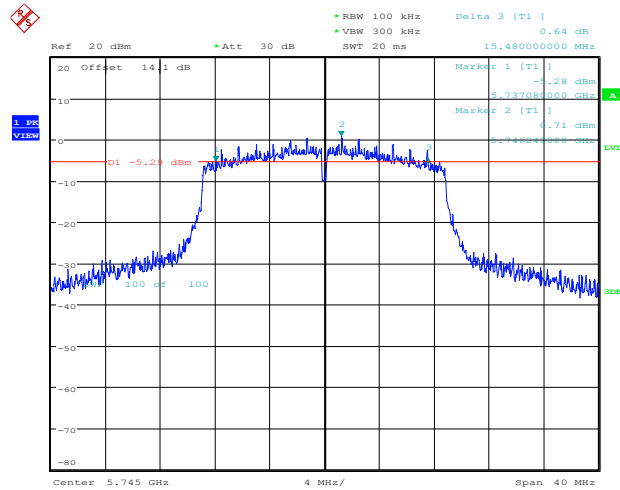
11N20SISO_Ant1_5745
