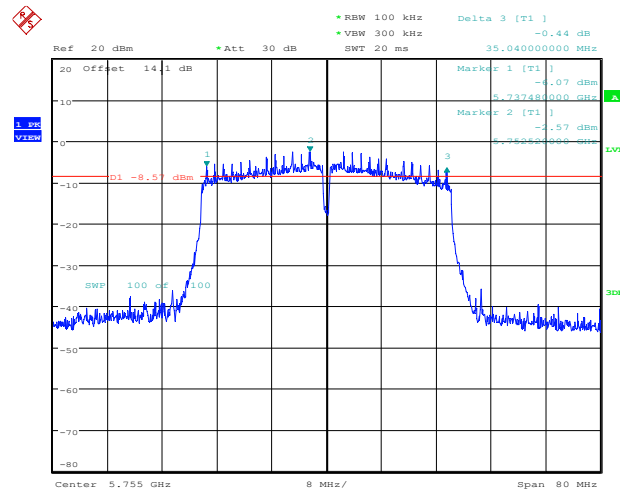
11AC40SISO_Ant1_5755
