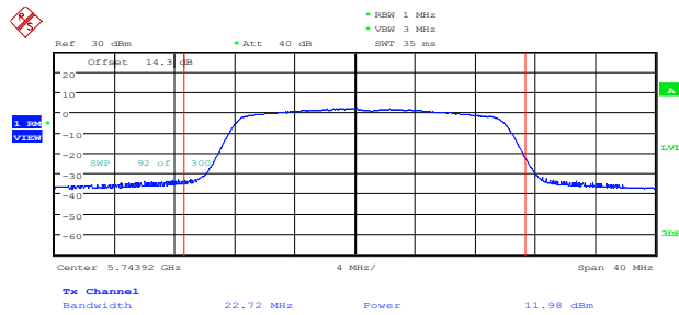
11N20SISO_Ant1_5745
