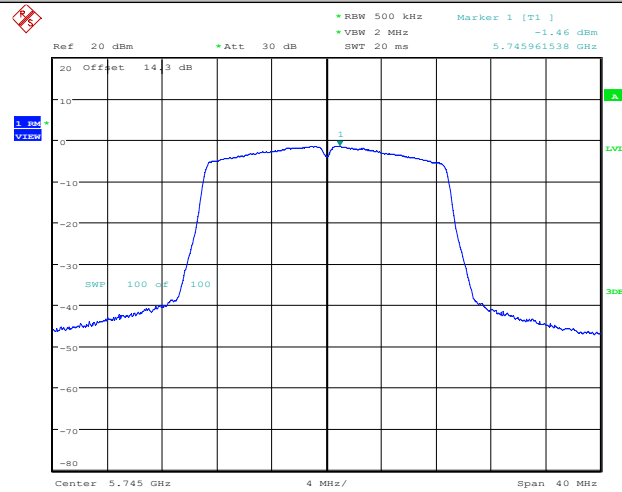
11N20SISO_Ant1_5745
