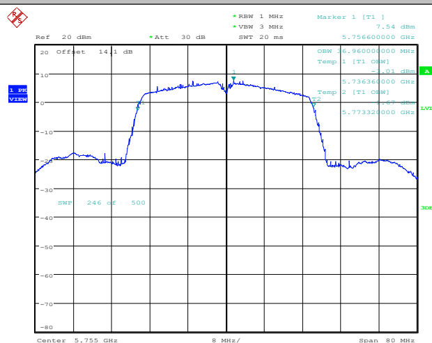
11N40SISO_Ant1_5755
