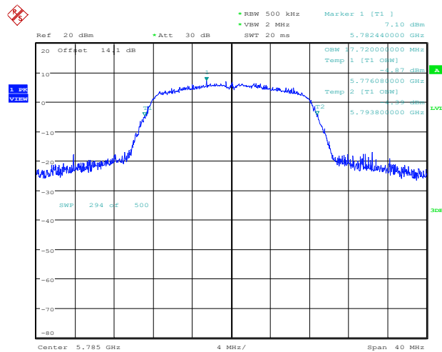
11A_Ant1_5785
