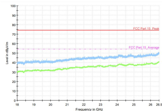
Radiated Spurious Emission (802.11ac 80m, ch106, 18GHz-26.5GHz)
