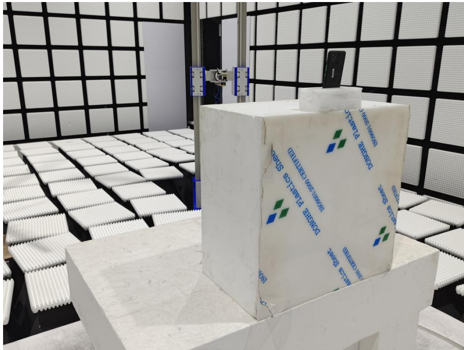
Description: Radiated Emission Test Setup (18GHz -26.5GHz)
