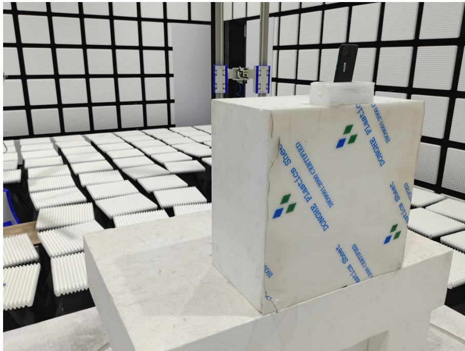
Description: Radiated Emission Test Setup (26.5GHz -40GHz)
